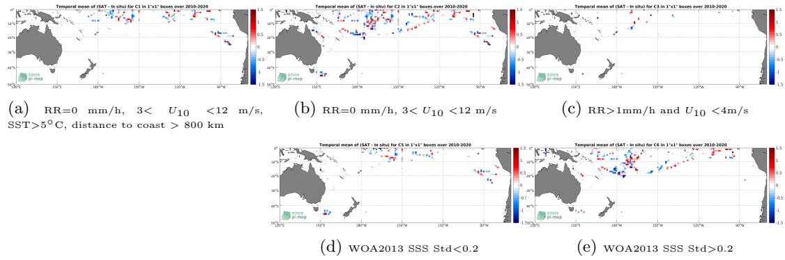
Figure 12: Temporal mean gridded over spatial boxes of size 1^\circ \times 1^\circ of \Delta SSS (SMOS SSS L2 v662 (ESA) - TSG (SAMOS)) for 5 different subdatasets corresponding to: RR=0 mm/h, 3 < U_{10} < 12 m/s, SST >5^\circ\text{C} , distance to coast > 800 km (a), RR=0 mm/h, 3 < U_{10} < 12 m/s (b), RR>1\text{mm/h} and U_{10} < 4\text{m/s} (c), WOA2013 SSS Std <0.2 (d), WOA2013 SSS Std >0.2 (e).
