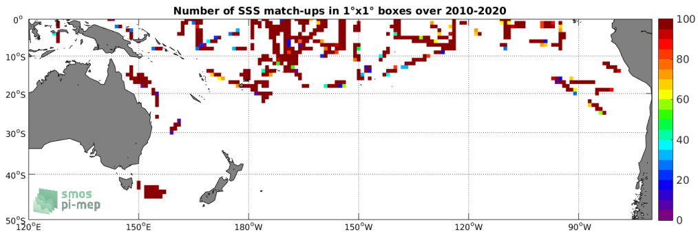
Figure 4: Number of SSS match-ups between TSG (SAMOS) SSS and the SMOS SSS L2 v662 (ESA) SSS product for the South Pacific Ocean Pi-MEP region over 1^\circ \times 1^\circ boxes and for the full satellite product period.
