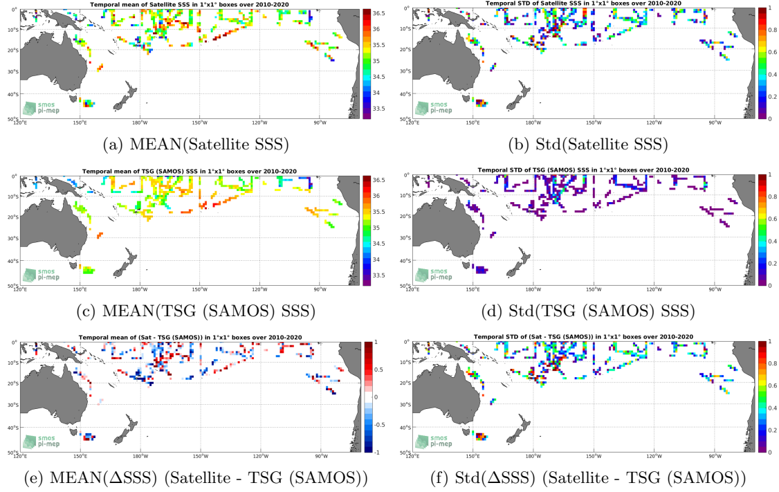
Figure 6: Temporal mean (left) and Std (right) of SSS from SMOS SSS L2 v662 (ESA) (top), TSG (SAMOS) (middle), and of \Delta SSS (Satellite - TSG (SAMOS)). Only match-up pairs are used to generate these maps.
