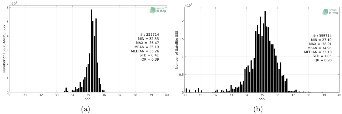
Figure 2: Histograms of SSS from TSG (SAMOS) (a) and SMOS SSS L2 v662 (ESA) (b) considering all match-up pairs per bins of 0.1 over the South Pacific Ocean Pi-MEP region and for the full satellite product period.
