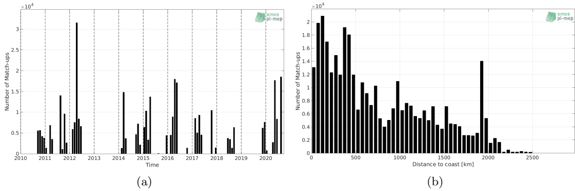
Figure 1: Number of match-ups between TSG (SAMOS) and SMOS SSS L2 v662 (ESA) SSS as a function of time (a) and as function of the distance to coast (b) over the South Pacific Ocean Pi-MEP region and for the full satellite product period.
