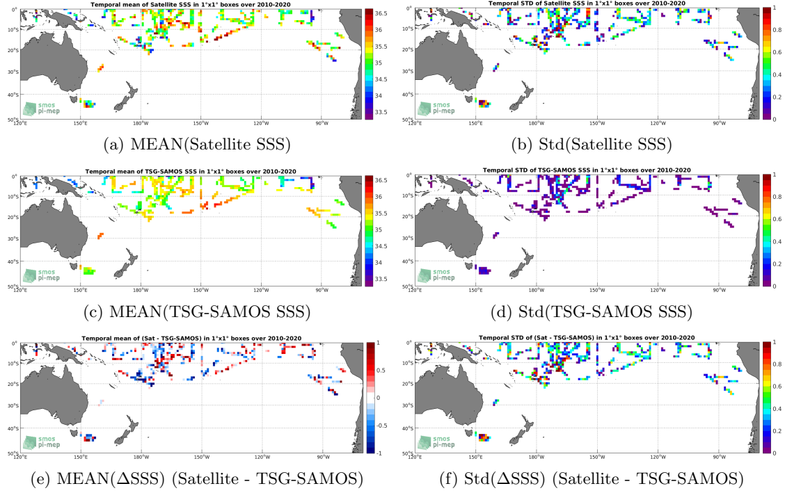
Figure 6: Temporal mean (left) and Std (right) of SSS from SMOS L2 v662 (ESA) (top), TSG-SAMOS (middle), and of \Delta SSS (Satellite - TSG-SAMOS). Only match-up pairs are used to generate these maps.
