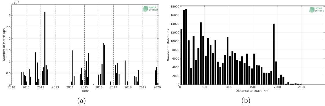
Figure 1: Number of match-ups between TSG-SAMOS and SMOS L2 v662 (ESA) SSS as a function of time (a) and as function of the distance to coast (b) over the South Pacific Ocean Pi-MEP region and for the full satellite product period.
