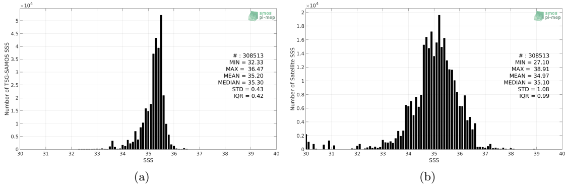
Figure 2: Histograms of SSS from TSG-SAMOS (a) and SMOS L2 v662 (ESA) (b) considering all match-up pairs per bins of 0.1 over the South Pacific Ocean Pi-MEP region and for the full satellite product period.
