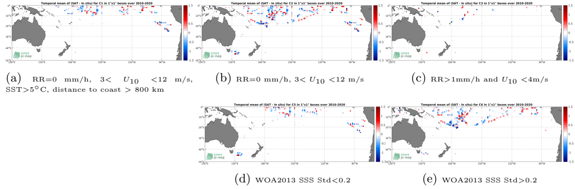
Figure 12: Temporal mean gridded over spatial boxes of size 1^\circ \times 1^\circ of \Delta SSS (SMOS L2 v662 (ESA) - TSG-SAMOS) for 5 different subdatasets corresponding to: RR=0 mm/h, 3 < U_{10} < 12 m/s, SST > 5^\circ C , distance to coast > 800 km (a), RR=0 mm/h, 3 < U_{10} < 12 m/s (b), RR > 1 mm/h and U_{10} < 4 m/s (c), WOA2013 SSS Std < 0.2 (d), WOA2013 SSS Std > 0.2 (e).
