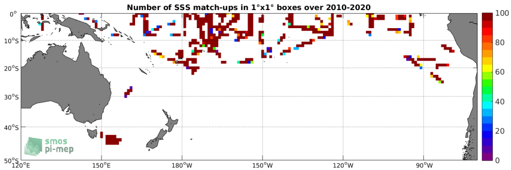
Figure 4: Number of SSS match-ups between TSG-SAMOS SSS and the SMOS L2 v662 (ESA) SSS product for the South Pacific Ocean Pi-MEP region over 1°x1° boxes and for the full satellite product period.
