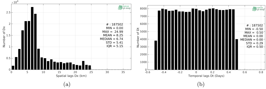
Figure 5: Histograms of the spatial (a) and temporal (b) lags between the time of the TSG-SAMOS measurements and the date of the corresponding SMOS-L2-DPGS-v662 SSS product.
