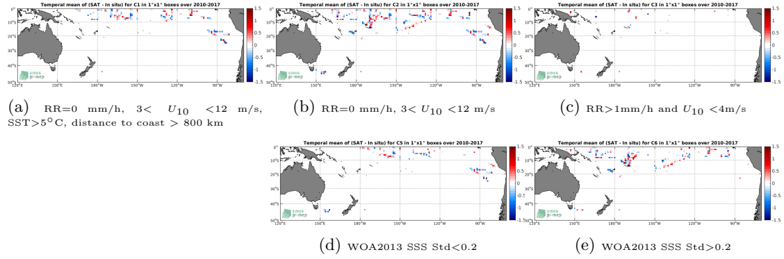
Figure 12: Temporal mean gridded over spatial boxes of size 1^\circ \times 1^\circ of \Delta SSS (SMOS-L2-DPGS-v662 - TSG-SAMOS) for 5 different subdatasets corresponding to: RR=0 mm/h, 3 < U_{10} < 12 m/s, SST > 5^\circ\text{C} , distance to coast > 800 km (a), RR=0 mm/h, 3 < U_{10} < 12 m/s (b), RR > 1 mm/h and U_{10} < 4 m/s (c), WOA2013 SSS Std < 0.2 (d), WOA2013 SSS Std > 0.2 (e).
