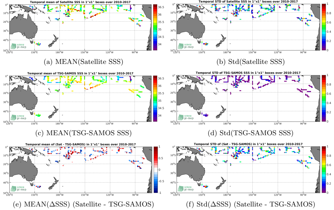
Figure 6: Temporal mean (left) and Std (right) of SSS from SMOS-L2-DPGS-v662 (top), TSG-SAMOS (middle), and of \Delta SSS (Satellite - TSG-SAMOS). Only match-up pairs are used to generate these maps.
