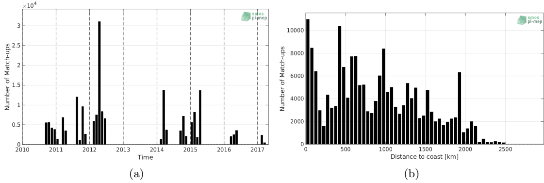
Figure 1: Number of match-ups between TSG-SAMOS and SMOS-L2-DPGS-v662 SSS as a function of time (a) and as function of the distance to coast (b) over the South Pacific Ocean Pi-MEP region and for the full satellite product period.
