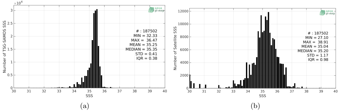
Figure 2: Histograms of SSS from TSG-SAMOS (a) and SMOS-L2-DPGS-v662 (b) considering all match-up pairs per bins of 0.1 over the South Pacific Ocean Pi-MEP region and for the full satellite product period.
