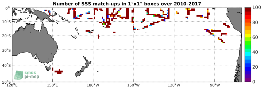
Figure 4: Number of SSS match-ups between TSG-SAMOS SSS and the SMOS-L2-DPGS-v662 SSS product for the South Pacific Ocean Pi-MEP region over 1°x1° boxes and for the full satellite product period.
