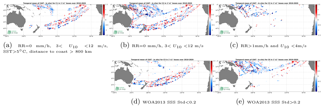
Figure 12: Temporal mean gridded over spatial boxes of size 1^\circ \times 1^\circ of \Delta SSS (SMOS SSS L2 v662 (ESA) - TSG (LEGOS-DM)) for 5 different subdatasets corresponding to:RR=0 mm/h, 3 < U_{10} < 12 m/s, SST >5^\circ C, distance to coast > 800 km (a), RR=0 mm/h, 3 < U_{10} < 12 m/s (b), RR >1 mm/h and U_{10} < 4 m/s (c), WOA2013 SSS Std <0.2 (d), WOA2013 SSS Std >0.2 (e).
