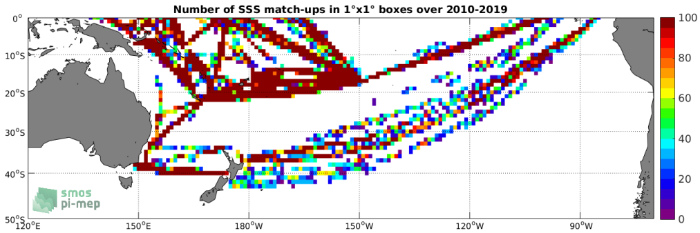
Figure 4: Number of SSS match-ups between TSG (LEGOS-DM) SSS and the SMOS SSS L2 v662 (ESA) SSS product for the South Pacific Ocean Pi-MEP region over 1^\circ \times 1^\circ boxes and for the full satellite product period.
