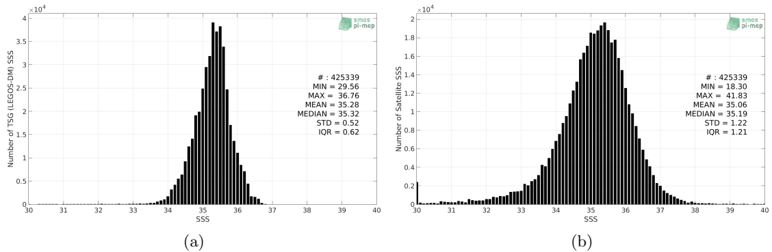
Figure 2: Histograms of SSS from TSG (LEGOS-DM) (a) and SMOS SSS L2 v662 (ESA) (b) considering all match-up pairs per bins of 0.1 over the South Pacific Ocean Pi-MEP region and for the full satellite product period.
