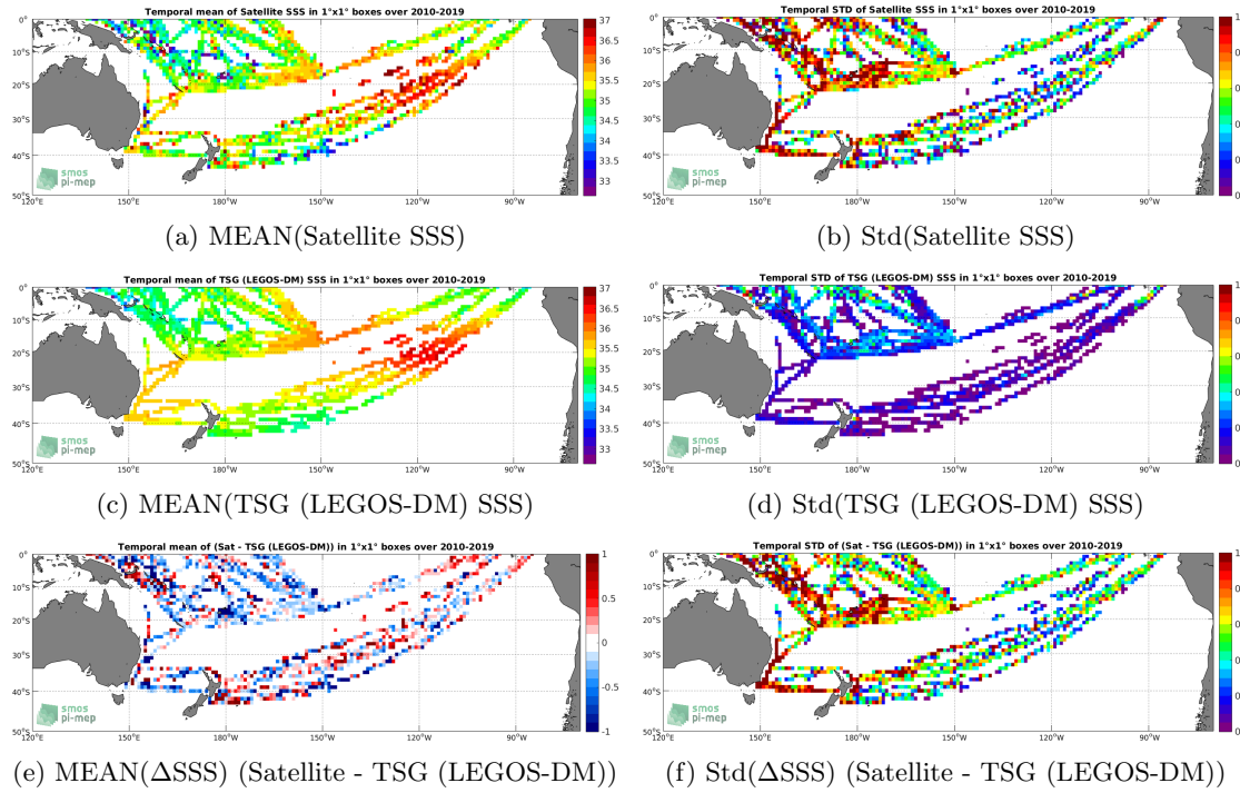
Figure 6: Temporal mean (left) and Std (right) of SSS from SMOS SSS L2 v662 (ESA) (top), TSG (LEGOS-DM) (middle), and of \Delta SSS (Satellite - TSG (LEGOS-DM)). Only match-up pairs are used to generate these maps.
