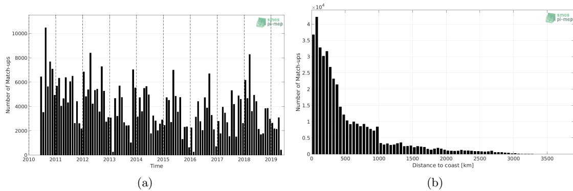
Figure 1: Number of match-ups between TSG (LEGOS-DM) and SMOS SSS L2 v662 (ESA) SSS as a function of time (a) and as function of the distance to coast (b) over the South Pacific Ocean Pi-MEP region and for the full satellite product period.
