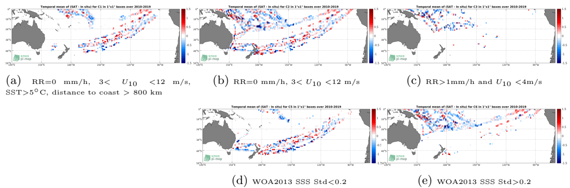
Figure 12: Temporal mean gridded over spatial boxes of size 1°x1° of \Delta SSS (SMOS SSS L2 v662 (ESA) - TSG (LEGOS-DM)) for 5 different subdatasets corresponding to:RR=0 mm/h, 3 < U_{10} < 12 m/s, SST>5°C, distance to coast > 800 km (a), RR=0 mm/h, 3 < U_{10} < 12 m/s (b), RR>1mm/h and U_{10} < 4 m/s (c), WOA2013 SSS Std<0.2 (d), WOA2013 SSS Std>0.2 (e).
