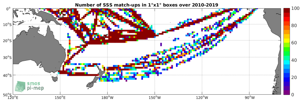
Figure 4: Number of SSS match-ups between TSG-LEGOS-DM SSS and the SMOS L2 v662 (ESA) SSS product for the South Pacific Ocean Pi-MEP region over 1°x1° boxes and for the full satellite product period.
