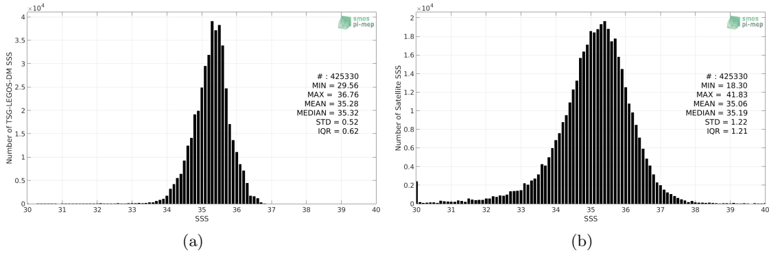
Figure 2: Histograms of SSS from TSG-LEGOS-DM (a) and SMOS L2 v662 (ESA) (b) considering all match-up pairs per bins of 0.1 over the South Pacific Ocean Pi-MEP region and for the full satellite product period.
