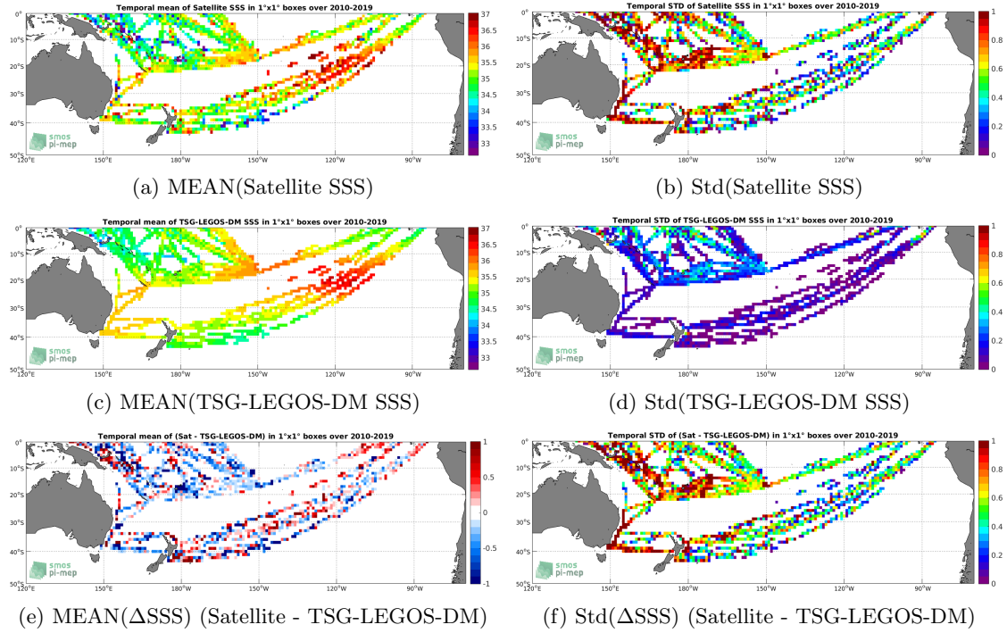
Figure 6: Temporal mean (left) and Std (right) of SSS from SMOS L2 v662 (ESA) (top), TSG-LEGOS-DM (middle), and of \Delta SSS (Satellite - TSG-LEGOS-DM). Only match-up pairs are used to generate these maps.
