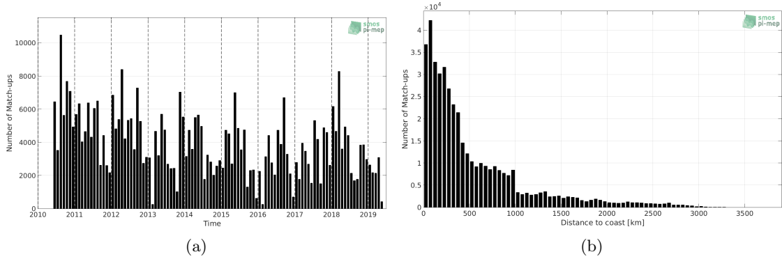
Figure 1: Number of match-ups between TSG-LEGOS-DM and SMOS L2 v662 (ESA) SSS as a function of time (a) and as function of the distance to coast (b) over the South Pacific Ocean Pi-MEP region and for the full satellite product period.
