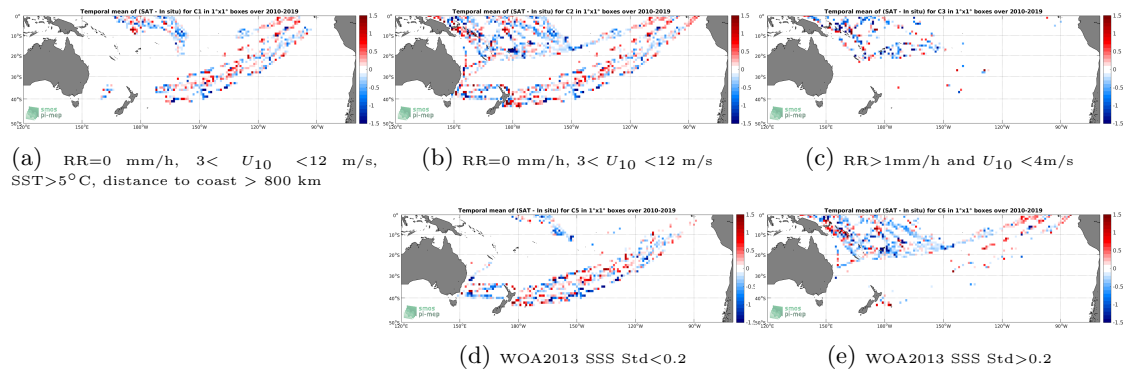
Figure 12: Temporal mean gridded over spatial boxes of size 1^\circ \times 1^\circ of \Delta SSS (SMOS L2 v662 (ESA) - TSG-LEGOS-DM) for 5 different subdatasets corresponding to:RR=0 mm/h, 3 < U_{10} < 12 m/s, SST >5^\circ\text{C} , distance to coast > 800 km (a), RR=0 mm/h, 3 < U_{10} < 12 m/s (b), RR >1 mm/h and U_{10} < 4 m/s (c), WOA2013 SSS Std <0.2 (d), WOA2013 SSS Std >0.2 (e).
