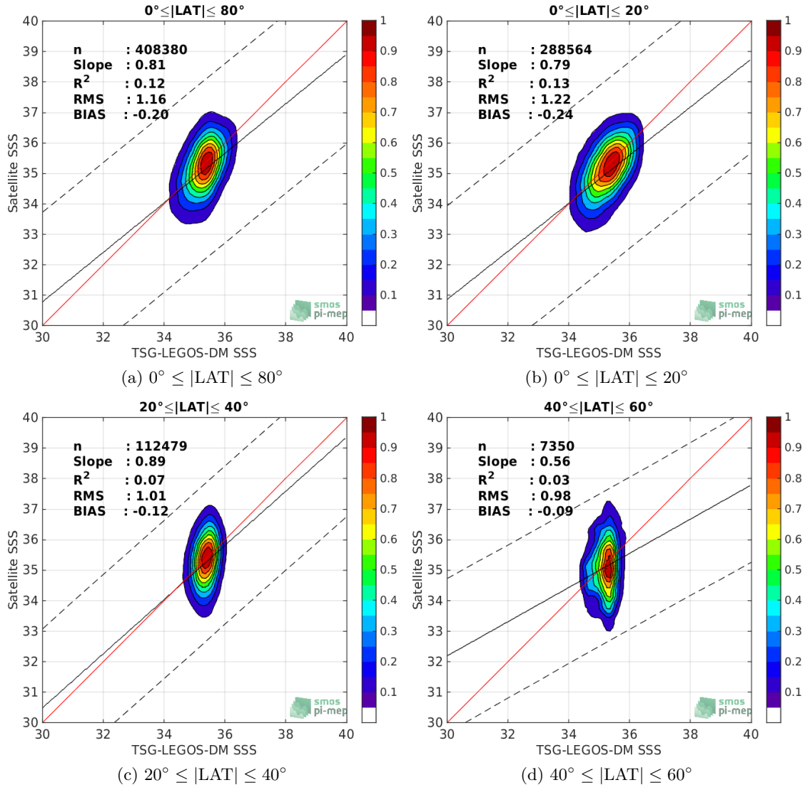
Figure 9: Contour maps of the concentration of SMOS-L2-DPGS-v662 SSS (y-axis) versus TSG-LEGOS-DM SSS (x-axis) at match-up pairs for different latitude bands. For each plot, the red line shows x=y . The black thin and dashed lines indicate a linear fit through the data cloud and the \pm 95\% confidence levels, respectively. The number match-up pairs n , the slope and R^2 coefficient of the linear fit, the root mean square (RMS) and the mean bias between satellite and in situ data are indicated for each latitude band in each plots.
