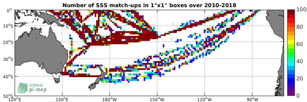
Figure 4: Number of SSS match-ups between TSG-LEGOS-DM SSS and the SMOS-L2-DPGS-v662 SSS product for the South Pacific Ocean Pi-MEP region over 1^\circ \times 1^\circ boxes and for the full satellite product period.
