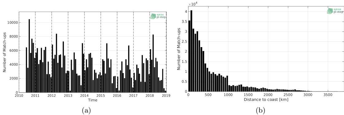
Figure 1: Number of match-ups between TSG-LEGOS-DM and SMOS-L2-DPGS-v662 SSS as a function of time (a) and as function of the distance to coast (b) over the South Pacific Ocean Pi-MEP region and for the full satellite product period.
