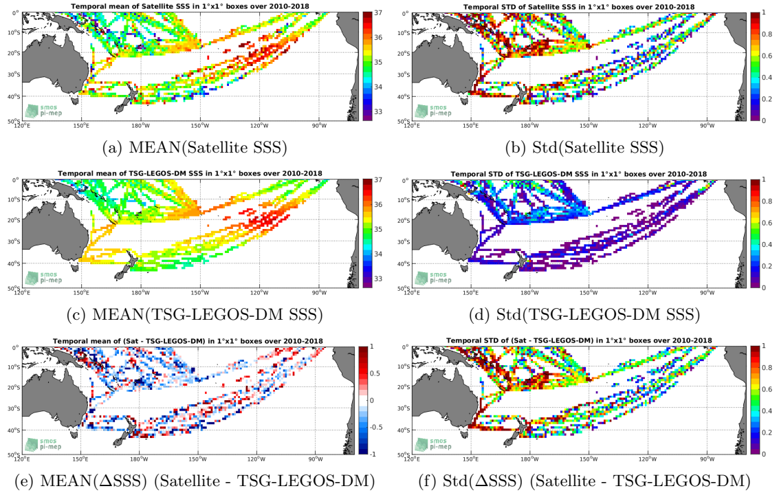
Figure 6: Temporal mean (left) and Std (right) of SSS from SMOS-L2-DPGS-v662 (top), TSG-LEGOS-DM (middle), and of \Delta SSS (Satellite - TSG-LEGOS-DM). Only match-up pairs are used to generate these maps.
