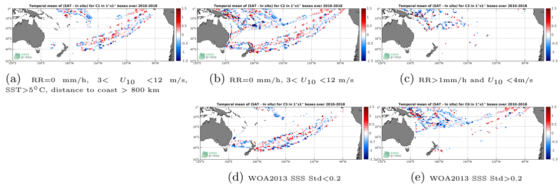
Figure 12: Temporal mean gridded over spatial boxes of size 1^\circ \times 1^\circ of \Delta SSS (SMOS-L2-DPGS-v662 - TSG-LEGOS-DM) for 5 different subdatasets corresponding to:RR=0 mm/h, 3 < U_{10} < 12 m/s, SST >5^\circ C, distance to coast > 800 km (a), RR=0 mm/h, 3 < U_{10} < 12 m/s (b), RR >1 mm/h and U_{10} < 4 m/s (c), WOA2013 SSS Std <0.2 (d), WOA2013 SSS Std >0.2 (e).
