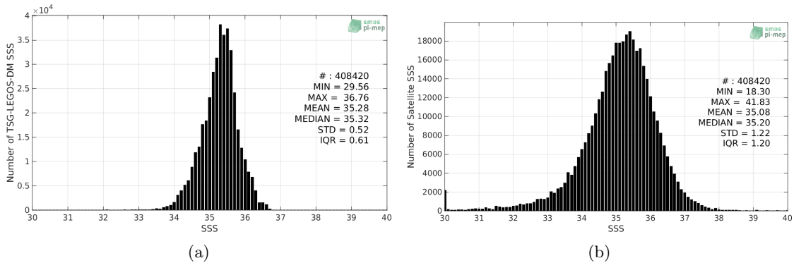
Figure 2: Histograms of SSS from TSG-LEGOS-DM (a) and SMOS-L2-DPGS-v662 (b) considering all match-up pairs per bins of 0.1 over the South Pacific Ocean Pi-MEP region and for the full satellite product period.
