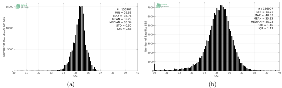
Figure 2: Histograms of SSS from TSG-LEGOS-DM (a) and SMOS-L2-DPGS-v662 (b) considering all match-up pairs per bins of 0.1 over the South Pacific Ocean Pi-MEP region and for the full satellite product period.
