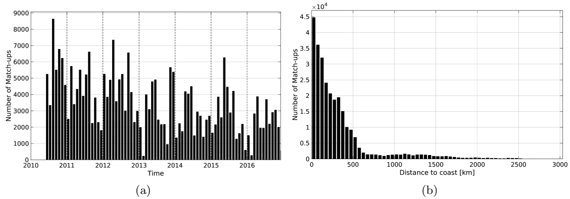
Figure 1: Number of match-ups between TSG-LEGOS-DM and SMOS-L2-DPGS-v662 SSS as a function of time (a) and as function of the distance to coast (b) over the South Pacific Ocean Pi-MEP region and for the full satellite product period.
