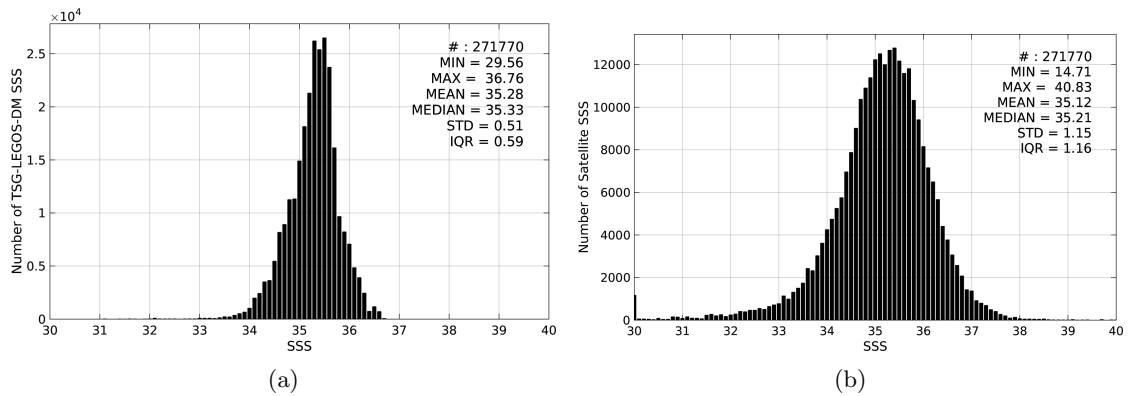
Figure 2: Histograms of SSS from TSG-LEGOS-DM (a) and SMOS-L2-DPGS-v662 (b) considering all match-up pairs per bins of 0.1 over the South Pacific Ocean Pi-MEP region and for the full satellite product period.
