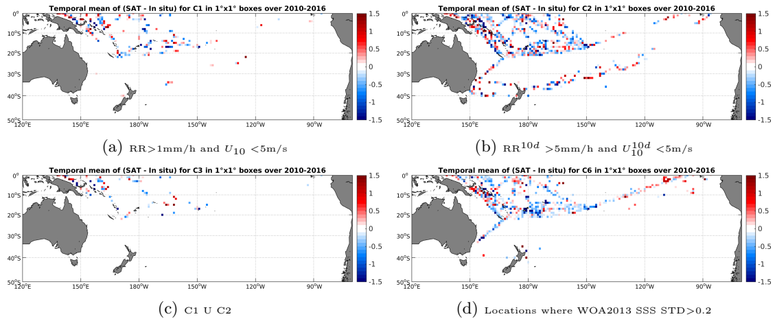
Figure 12: Temporal mean gridded over spatial boxes of size 1^\circ \times 1^\circ of \Delta SSS (SMOS-L2-DPGS-v662 - TSG-LEGOS-DM) for 4 different subdatasets corresponding to:RR >1 mm/h and U_{10} < 5 m/s (a), RR 10d > 5 mm/h and U_{10}^{10d} < 5 m/s (b), C1 U C2 (c),Locations where WOA2013 SSS STD >0.2 (d).
