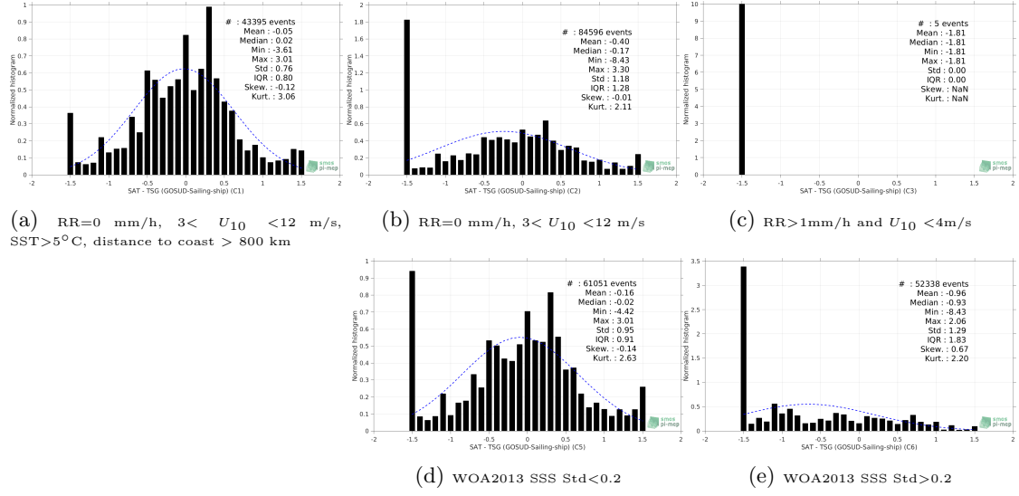
Figure 13: Normalized histogram of \Delta SSS (SMOS SSS L2 v662 (ESA) - TSG (GOSUD-Sailing-ship)) for 5 different subdatasets corresponding to: RR=0 mm/h, 3 < U_{10} < 12 m/s, SST>5°C, distance to coast > 800 km (a), RR=0 mm/h, 3 < U_{10} < 12 m/s (b), RR>1mm/h and U_{10} < 4 m/s (c), WOA2013 SSS Std<0.2 (d), WOA2013 SSS Std>0.2 (e).
