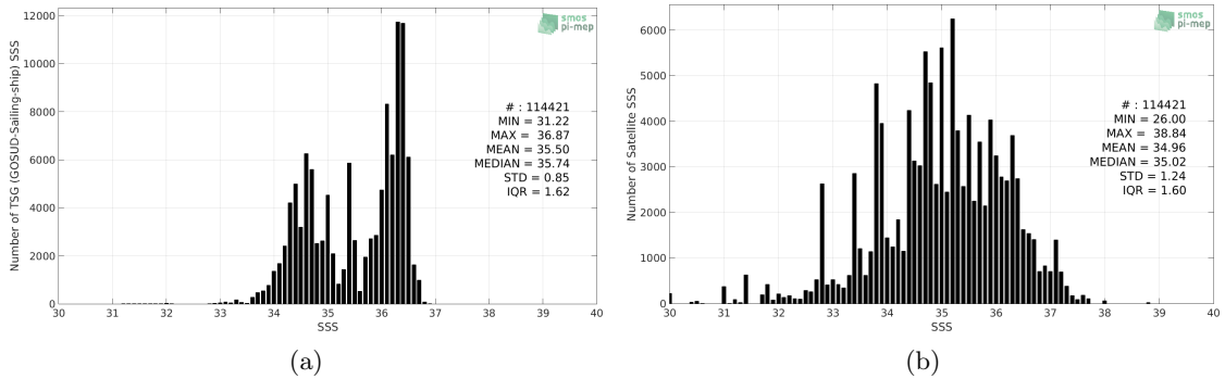
Figure 2: Histograms of SSS from TSG (GOSUD-Sailing-ship) (a) and SMOS SSS L2 v662 (ESA) (b) considering all match-up pairs per bins of 0.1 over the South Pacific Ocean Pi-MEP region and for the full satellite product period.
