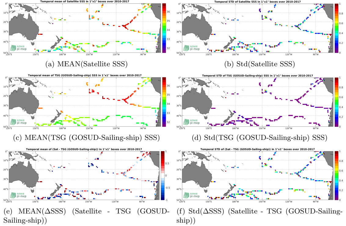
Figure 6: Temporal mean (left) and Std (right) of SSS from SMOS SSS L2 v662 (ESA) (top), TSG (GOSUD-Sailing-ship) (middle), and of \Delta SSS (Satellite - TSG (GOSUD-Sailing-ship)). Only match-up pairs are used to generate these maps.
