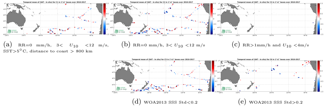
Figure 12: Temporal mean gridded over spatial boxes of size 1^\circ \times 1^\circ of \Delta SSS (SMOS SSS L2 v662 (ESA) - TSG (GOSUD-Sailing-ship)) for 5 different subdatasets corresponding to: RR=0 mm/h, 3 < U_{10} < 12 m/s, SST > 5^\circ C , distance to coast > 800 km (a), RR=0 mm/h, 3 < U_{10} < 12 m/s (b), RR > 1 mm/h and U_{10} < 4 m/s (c), WOA2013 SSS Std < 0.2 (d), WOA2013 SSS Std > 0.2 (e).
