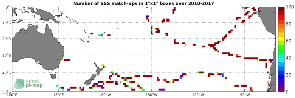
Figure 4: Number of SSS match-ups between TSG (GOSUD-Sailing-ship) SSS and the SMOS SSS L2 v662 (ESA) SSS product for the South Pacific Ocean Pi-MEP region over 1^\circ \times 1^\circ boxes and for the full satellite product period.
