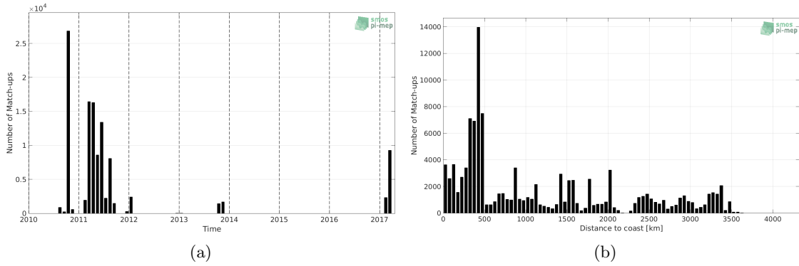
Figure 1: Number of match-ups between TSG (GOSUD-Sailing-ship) and SMOS SSS L2 v662 (ESA) SSS as a function of time (a) and as function of the distance to coast (b) over the South Pacific Ocean Pi-MEP region and for the full satellite product period.
