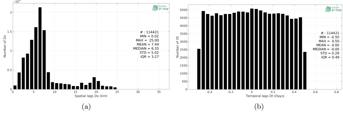
Figure 5: Histograms of the spatial (a) and temporal (b) lags between the time of the TSG (GOSUD-Sailing-ship) measurements and the date of the corresponding SMOS SSS L2 v662 (ESA) SSS product.
