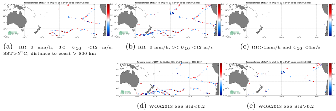
Figure 12: Temporal mean gridded over spatial boxes of size 1^\circ \times 1^\circ of \Delta SSS (SMOS L2 v662 (ESA) - TSG-GOSUD-Sailing-ship) for 5 different subdatasets corresponding to: RR=0 mm/h, 3 < U_{10} < 12 m/s, SST > 5^\circ\text{C} , distance to coast > 800 km (a), RR=0 mm/h, 3 < U_{10} < 12 m/s (b), RR > 1 mm/h and U_{10} < 4 m/s (c), WOA2013 SSS Std < 0.2 (d), WOA2013 SSS Std > 0.2 (e).
