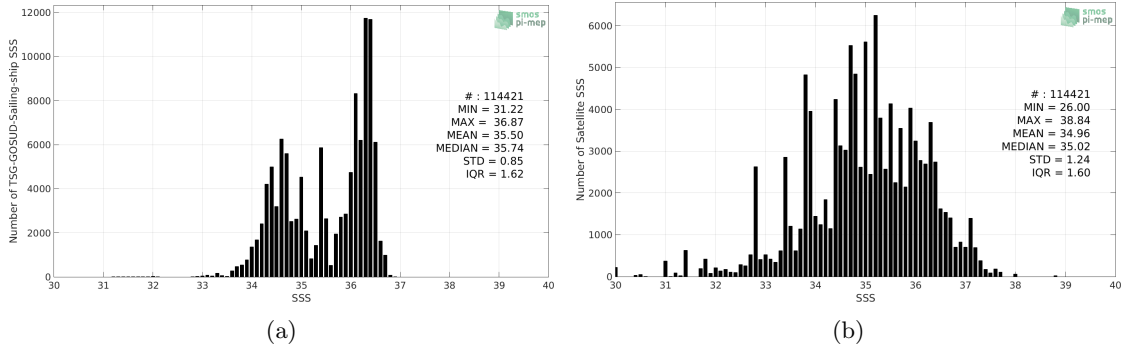
Figure 2: Histograms of SSS from TSG-GOSUD-Sailing-ship (a) and SMOS L2 v662 (ESA) (b) considering all match-up pairs per bins of 0.1 over the South Pacific Ocean Pi-MEP region and for the full satellite product period.
