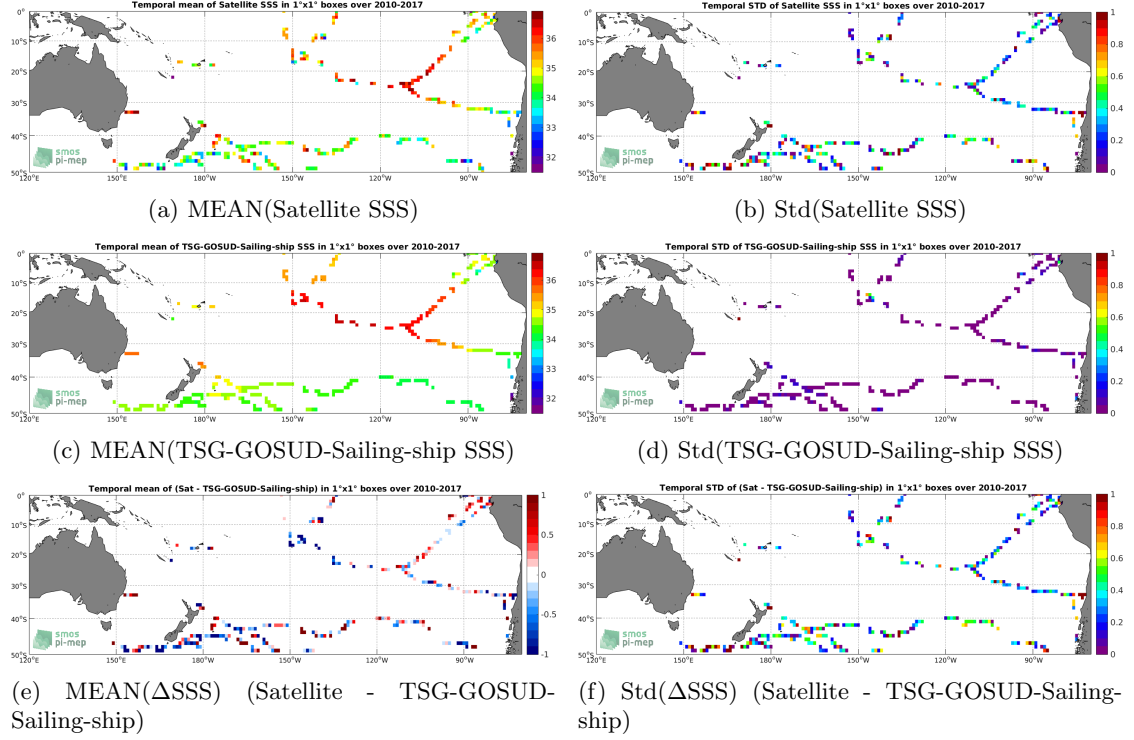
Figure 6: Temporal mean (left) and Std (right) of SSS from SMOS L2 v662 (ESA) (top), TSG-GOSUD-Sailing-ship (middle), and of \Delta SSS (Satellite - TSG-GOSUD-Sailing-ship). Only match-up pairs are used to generate these maps.
