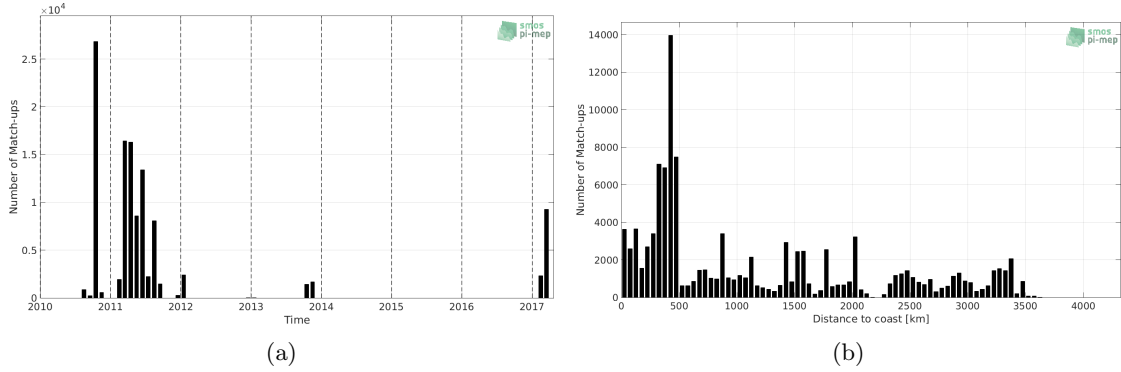
Figure 1: Number of match-ups between TSG-GOSUD-Sailing-ship and SMOS L2 v662 (ESA) SSS as a function of time (a) and as function of the distance to coast (b) over the South Pacific Ocean Pi-MEP region and for the full satellite product period.
