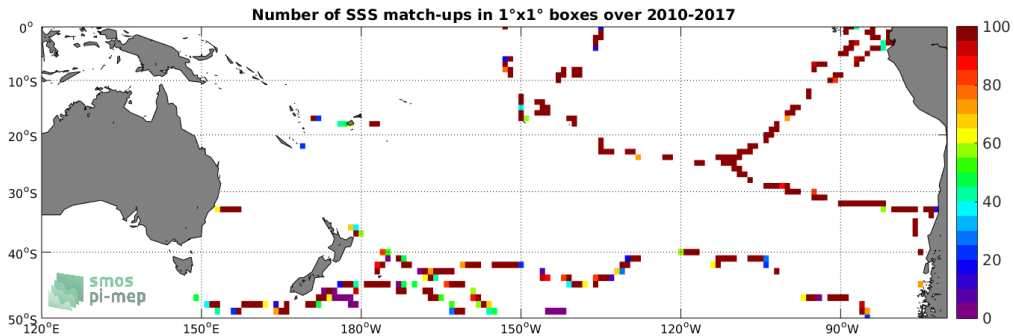
Figure 4: Number of SSS match-ups between TSG-GOSUD-Sailing-ship SSS and the SMOS L2 v662 (ESA) SSS product for the South Pacific Ocean Pi-MEP region over 1^\circ \times 1^\circ boxes and for the full satellite product period.
