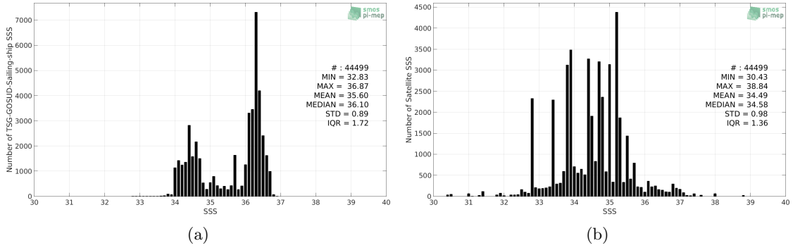
Figure 2: Histograms of SSS from TSG-GOSUD-Sailing-ship (a) and SMOS-L2-DPGS-v662 (b) considering all match-up pairs per bins of 0.1 over the South Pacific Ocean Pi-MEP region and for the full satellite product period.
