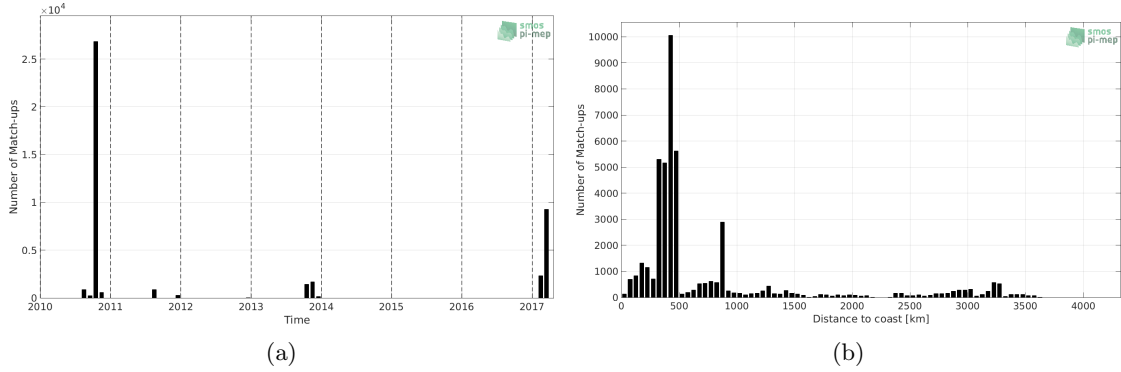
Figure 1: Number of match-ups between TSG-GOSUD-Sailing-ship and SMOS-L2-DPGS-v662 SSS as a function of time (a) and as function of the distance to coast (b) over the South Pacific Ocean Pi-MEP region and for the full satellite product period.
