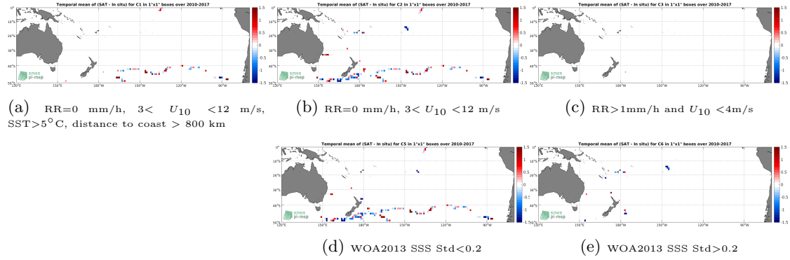
Figure 12: Temporal mean gridded over spatial boxes of size 1^\circ \times 1^\circ of \Delta SSS (SMOS-L2-DPGS-v662 - TSG-GOSUD-Sailing-ship) for 5 different subdatasets corresponding to: RR=0 mm/h, 3 < U_{10} < 12 m/s, SST > 5^\circ\text{C} , distance to coast > 800 km (a), RR=0 mm/h, 3 < U_{10} < 12 m/s (b), RR > 1 mm/h and U_{10} < 4 m/s (c), WOA2013 SSS Std < 0.2 (d), WOA2013 SSS Std > 0.2 (e).
