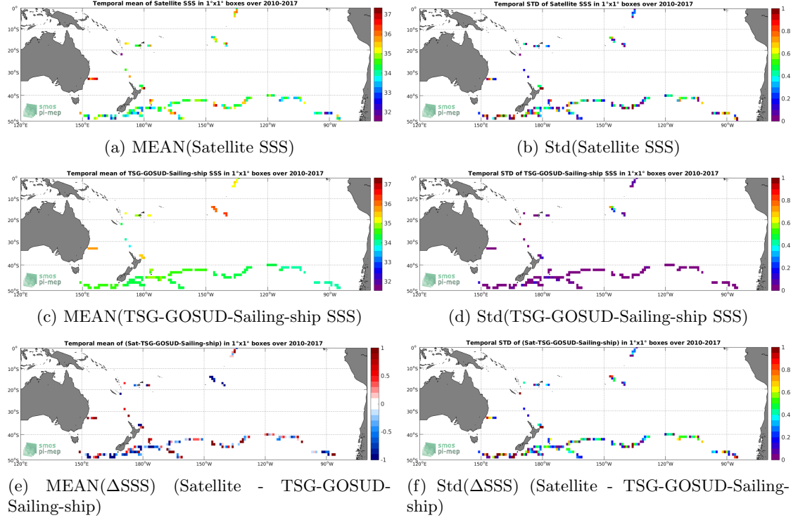
Figure 6: Temporal mean (left) and Std (right) of SSS from SMOS-L2-DPGS-v662 (top), TSG-GOSUD-Sailing-ship (middle), and of \Delta SSS (Satellite - TSG-GOSUD-Sailing-ship). Only match-up pairs are used to generate these maps.
