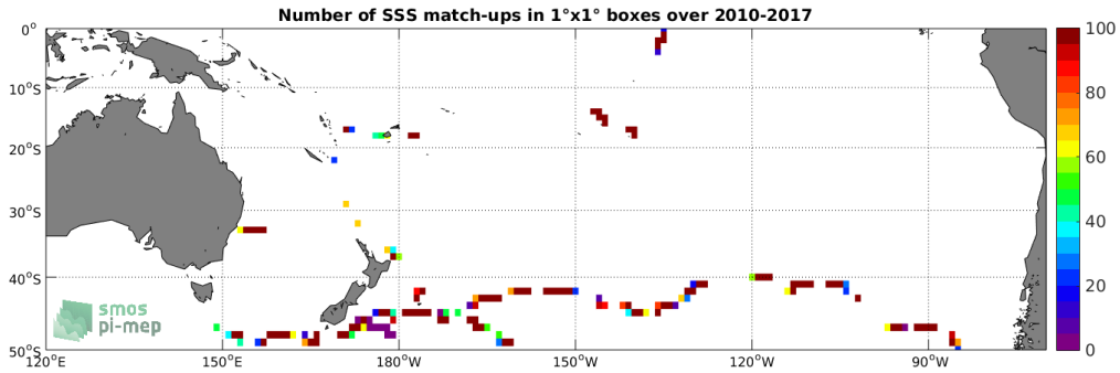
Figure 4: Number of SSS match-ups between TSG-GOSUD-Sailing-ship SSS and the SMOS-L2-DPGS-v662 SSS product for the South Pacific Ocean Pi-MEP region over 1^\circ \times 1^\circ boxes and for the full satellite product period.
