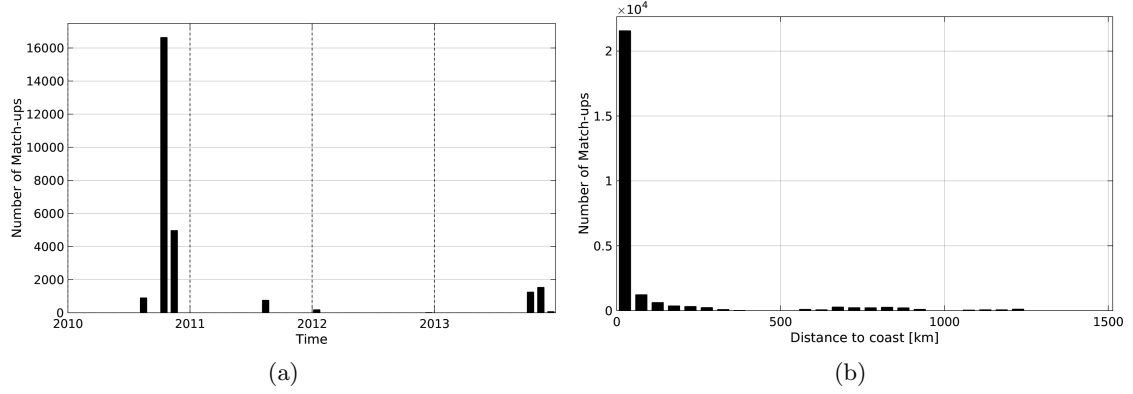
Figure 1: Number of match-ups between TSG-GOSUD-Sailing-ship and SMOS-L2-DPGS-v662 SSS as a function of time (a) and as function of the distance to coast (b) over the South Pacific Ocean Pi-MEP region and for the full satellite product period.
