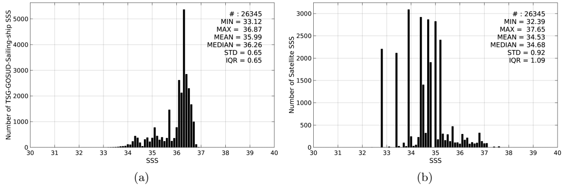
Figure 2: Histograms of SSS from TSG-GOSUD-Sailing-ship (a) and SMOS-L2-DPGS-v662 (b) considering all match-up pairs per bins of 0.1 over the South Pacific Ocean Pi-MEP region and for the full satellite product period.
