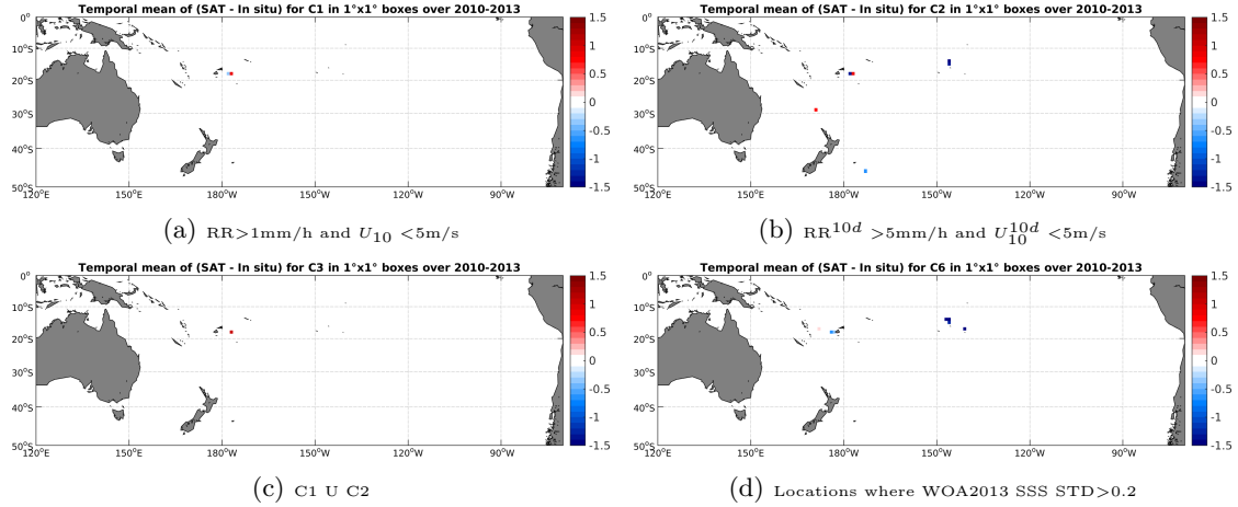
Figure 12: Temporal mean gridded over spatial boxes of size 1^\circ \times 1^\circ of \Delta SSS (SMOS-L2-DPGS-v662 - TSG-GOSUD-Sailing-ship) for 4 different subdatasets corresponding to: RR > 1\text{mm/h} and U_{10} < 5\text{m/s} (a), RR^{10d} > 5\text{mm/h} and U_{10}^{10d} < 5\text{m/s} (b), C1 U C2 (c), Locations where WOA2013 SSS STD > 0.2 (d).
