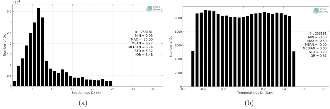
Figure 5: Histograms of the spatial (a) and temporal (b) lags between the location/time of the TSG (GOSUD-Research-vessel) measurement and the date of the corresponding SMOS SSS L2 v662 (ESA) SSS pixel.
