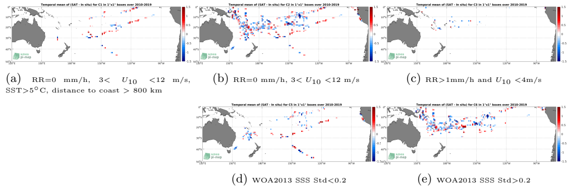
Figure 12: Temporal mean gridded over spatial boxes of size 1^\circ \times 1^\circ of \Delta SSS (SMOS SSS L2 v662 (ESA) - TSG (GOSUD-Research-vessel)) for 5 different subdatasets corresponding to: RR=0 mm/h, 3 < U_{10} < 12 m/s, SST > 5^\circ\text{C} , distance to coast > 800 km (a), RR=0 mm/h, 3 < U_{10} < 12 m/s (b), RR > 1 mm/h and U_{10} < 4 m/s (c), WOA2013 SSS Std < 0.2 (d), WOA2013 SSS Std > 0.2 (e).
