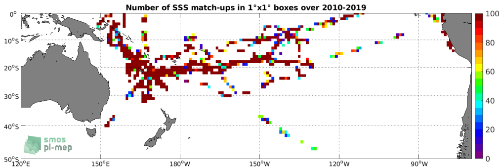
Figure 4: Number of SSS match-ups between TSG (GOSUD-Research-vessel) SSS and the SMOS SSS L2 v662 (ESA) SSS product for the South Pacific Ocean Pi-MEP region over 1^\circ \times 1^\circ boxes and for the full satellite product period.
