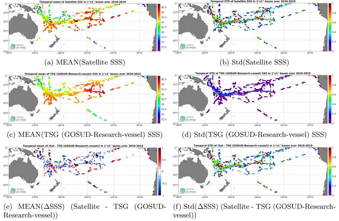
Figure 6: Temporal mean (left) and Std (right) of SSS from SMOS SSS L2 v662 (ESA) (top), TSG (GOSUD-Research-vessel) (middle), and of \Delta SSS (Satellite - TSG (GOSUD-Research-vessel)). Only match-up pairs are used to generate these maps.
