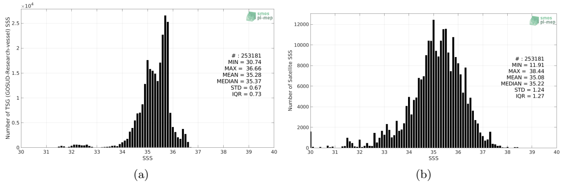
Figure 2: Histograms of SSS from TSG (GOSUD-Research-vessel) (a) and SMOS SSS L2 v662 (ESA) (b) considering all match-up pairs per bins of 0.1 over the South Pacific Ocean Pi-MEP region and for the full satellite product period.
