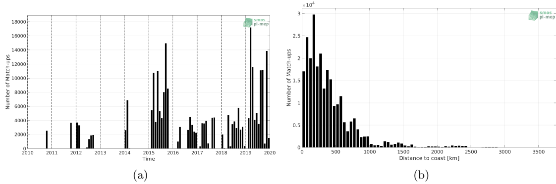
Figure 1: Number of match-ups between TSG (GOSUD-Research-vessel) and SMOS SSS L2 v662 (ESA) SSS as a function of time (a) and as function of the distance to coast (b) over the South Pacific Ocean Pi-MEP region and for the full satellite product period.
