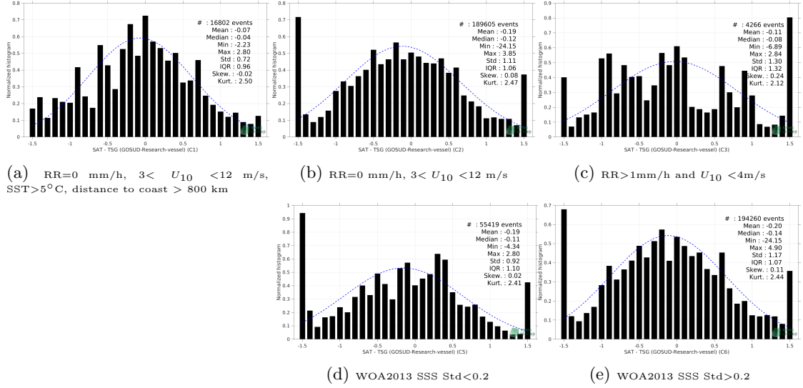
Figure 13: Normalized histogram of \Delta SSS (SMOS SSS L2 v662 (ESA) - TSG (GOSUD-Research-vessel)) for 5 different subdatasets corresponding to: RR=0 mm/h, 3 < U_{10} < 12 m/s, SST>5°C, distance to coast > 800 km (a), RR=0 mm/h, 3 < U_{10} < 12 m/s (b), RR>1mm/h and U_{10} < 4 m/s (c), WOA2013 SSS Std<0.2 (d), WOA2013 SSS Std>0.2 (e).
