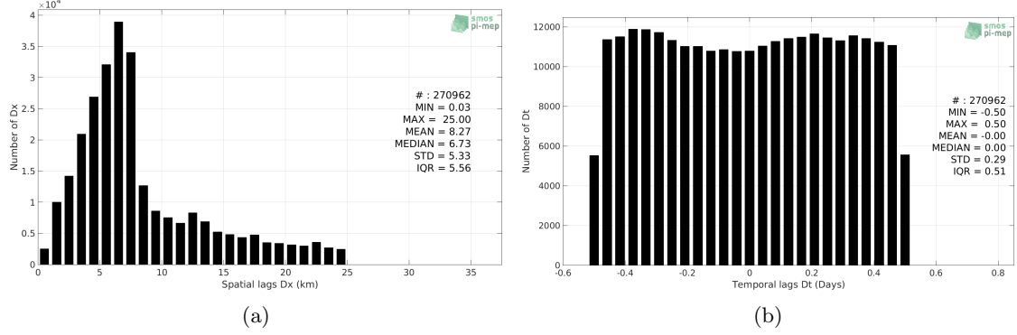
Figure 5: Histograms of the spatial (a) and temporal (b) lags between the time of the TSG (GOSUD-Research-vessel) measurements and the date of the corresponding SMOS SSS L2 v662 (ESA) SSS product.
