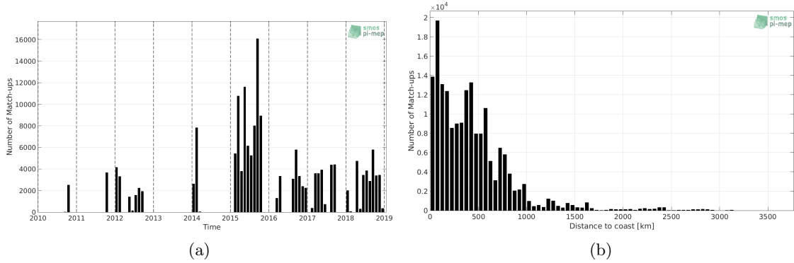
Figure 1: Number of match-ups between TSG-GOSUD-Research-vessel and SMOS L2 v662 (ESA) SSS as a function of time (a) and as function of the distance to coast (b) over the South Pacific Ocean Pi-MEP region and for the full satellite product period.
