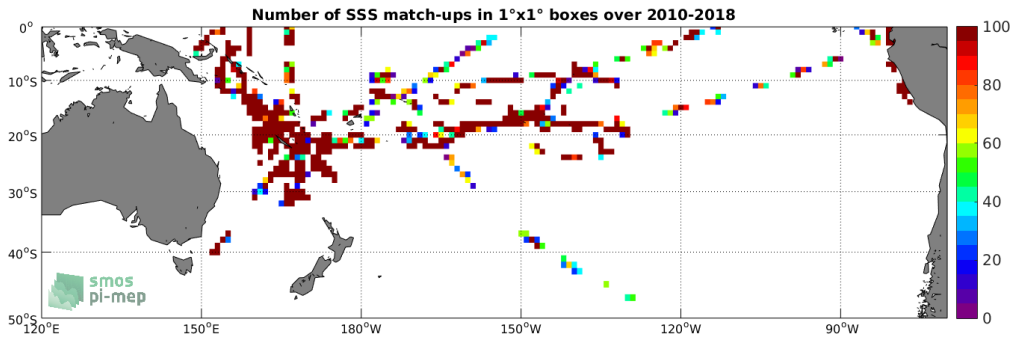
Figure 4: Number of SSS match-ups between TSG-GOSUD-Research-vessel SSS and the SMOS L2 v662 (ESA) SSS product for the South Pacific Ocean Pi-MEP region over 1^\circ \times 1^\circ boxes and for the full satellite product period.
