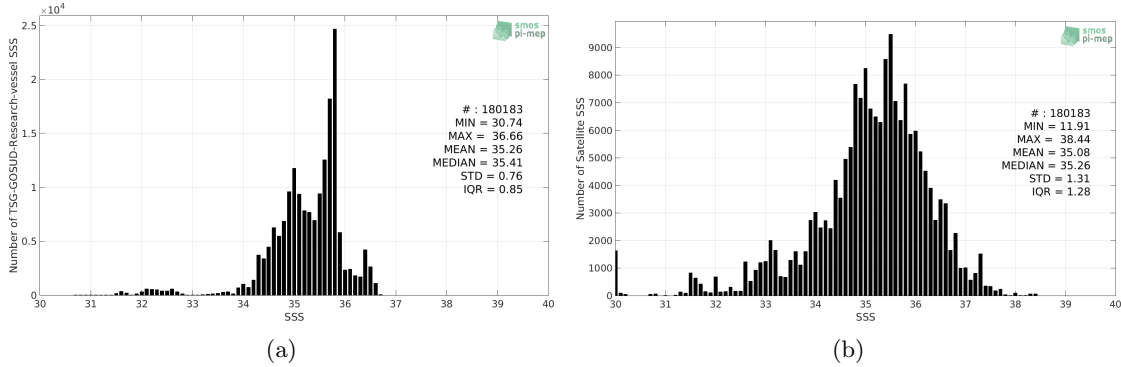
Figure 2: Histograms of SSS from TSG-GOSUD-Research-vessel (a) and SMOS L2 v662 (ESA) (b) considering all match-up pairs per bins of 0.1 over the South Pacific Ocean Pi-MEP region and for the full satellite product period.
