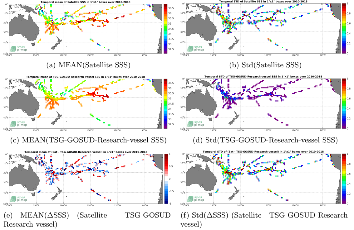
Figure 6: Temporal mean (left) and Std (right) of SSS from SMOS L2 v662 (ESA) (top), TSG-GOSUD-Research-vessel (middle), and of \Delta SSS (Satellite - TSG-GOSUD-Research-vessel). Only match-up pairs are used to generate these maps.
