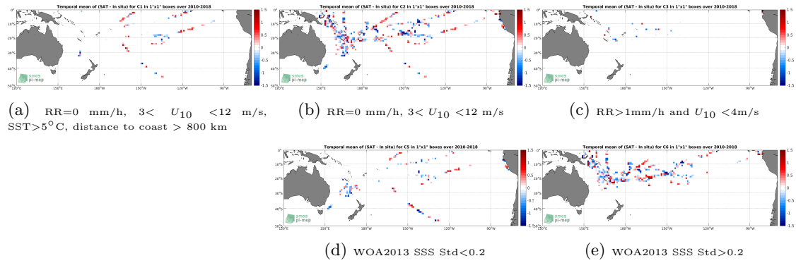
Figure 12: Temporal mean gridded over spatial boxes of size 1^\circ \times 1^\circ of \Delta SSS (SMOS L2 v662 (ESA) - TSG-GOSUD-Research-vessel) for 5 different subdatasets corresponding to: RR=0 mm/h, 3 < U_{10} < 12 m/s, SST > 5^\circ C , distance to coast > 800 km (a), RR=0 mm/h, 3 < U_{10} < 12 m/s (b), RR > 1 mm/h and U_{10} < 4 m/s (c), WOA2013 SSS Std < 0.2 (d), WOA2013 SSS Std > 0.2 (e).
