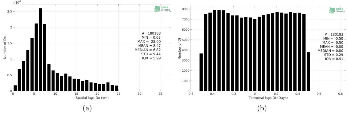
Figure 5: Histograms of the spatial (a) and temporal (b) lags between the time of the TSG-GOSUD-Research-vessel measurements and the date of the corresponding SMOS L2 v662 (ESA) SSS product.
