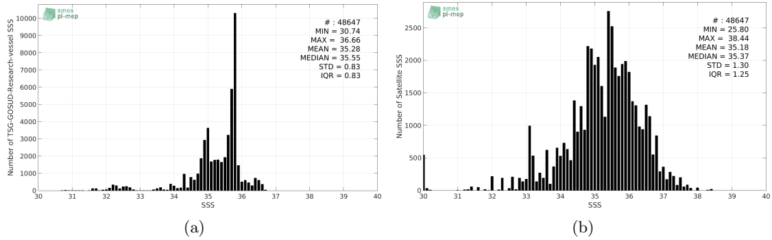
Figure 2: Histograms of SSS from TSG-GOSUD-Research-vessel (a) and SMOS-L2-DPGS-v662 (b) considering all match-up pairs per bins of 0.1 over the South Pacific Ocean Pi-MEP region and for the full satellite product period.
