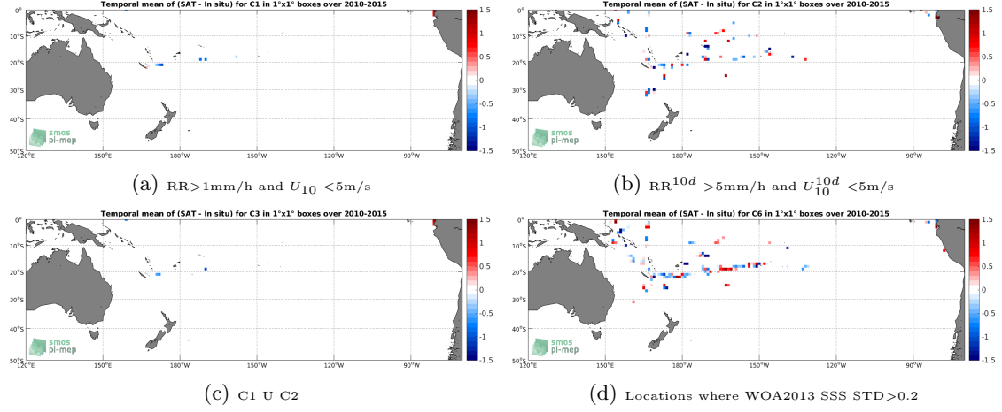
Figure 12: Temporal mean gridded over spatial boxes of size 1^\circ \times 1^\circ of \Delta SSS (SMOS-L2-DPGS-v662 - TSG-GOSUD-Research-vessel) for 4 different subdatasets corresponding to: RR > 1\text{mm/h} and U_{10} < 5\text{m/s} (a), RR^{10d} > 5\text{mm/h} and U_{10}^{10d} < 5\text{m/s} (b), C1 U C2 (c), Locations where WOA2013 SSS STD > 0.2 (d).
