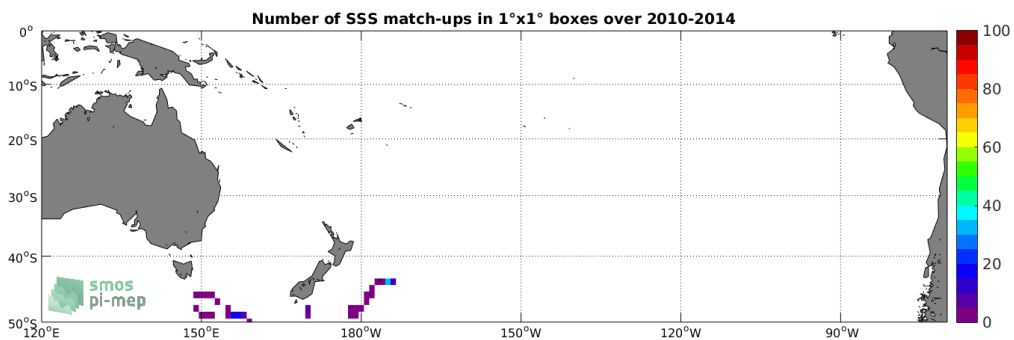
Figure 4: Number of SSS match-ups between Sea mammals SSS and the SMOS L2 v662 (ESA) SSS product for the South Pacific Ocean Pi-MEP region over 1^\circ \times 1^\circ boxes and for the full satellite product period.
