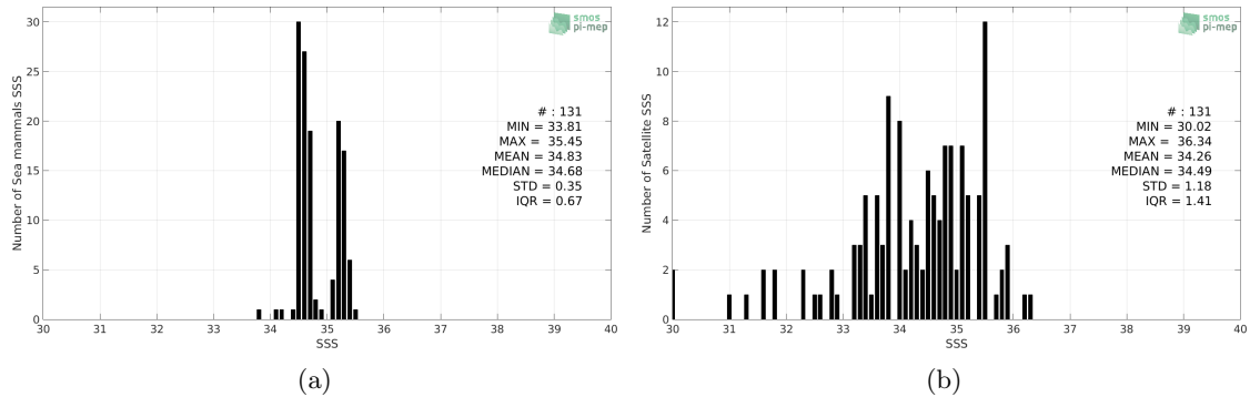
Figure 2: Histograms of SSS from Sea mammals (a) and SMOS L2 v662 (ESA) (b) considering all match-up pairs per bins of 0.1 over the South Pacific Ocean Pi-MEP region and for the full satellite product period.
