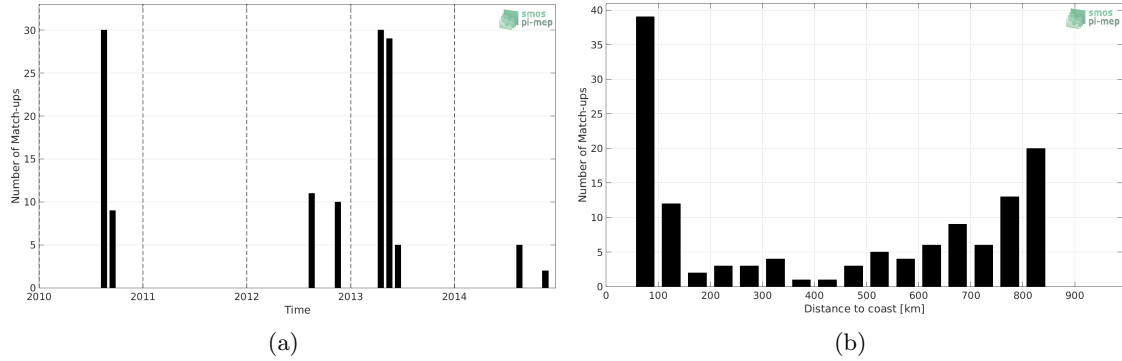
Figure 1: Number of match-ups between Sea mammals and SMOS L2 v662 (ESA) SSS as a function of time (a) and as function of the distance to coast (b) over the South Pacific Ocean Pi-MEP region and for the full satellite product period.
