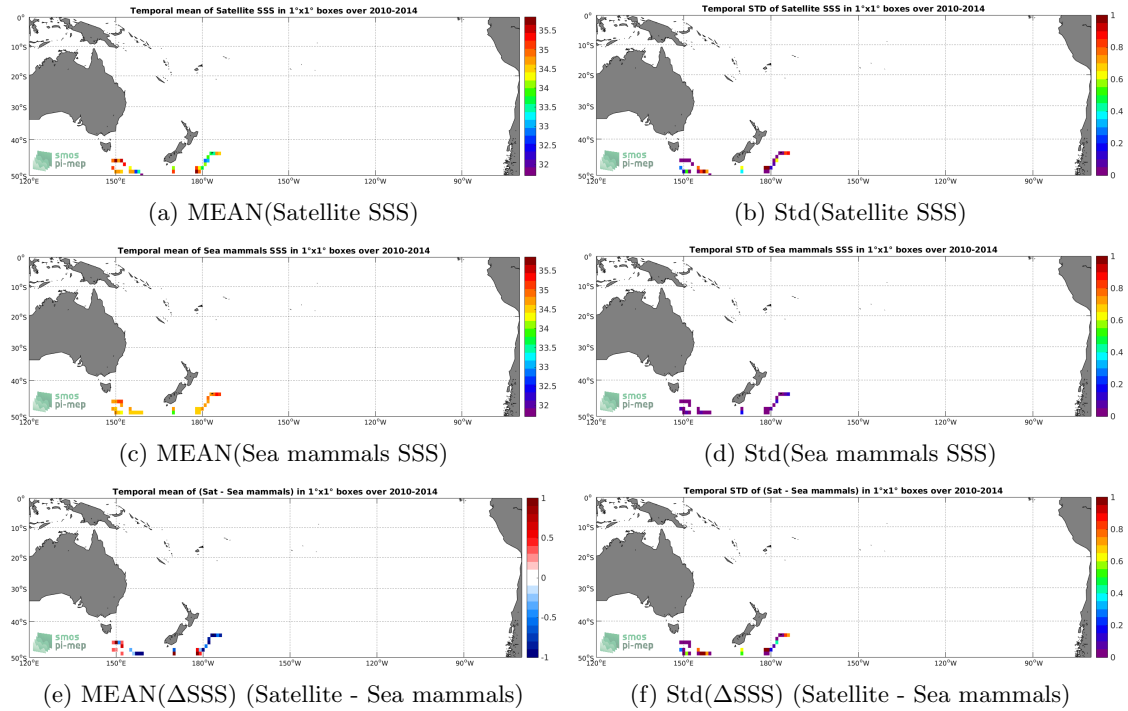
Figure 6: Temporal mean (left) and Std (right) of SSS from SMOS L2 v662 (ESA) (top), Sea mammals (middle), and of \Delta SSS (Satellite - Sea mammals). Only match-up pairs are used to generate these maps.
