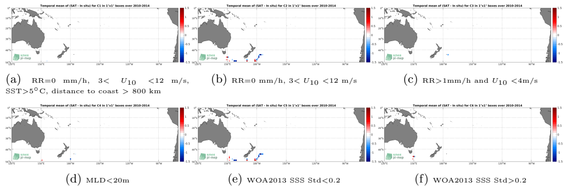
Figure 12: Temporal mean gridded over spatial boxes of size 1^{\circ}\times 1^{\circ} of \Delta\text{SSS} (SMOS L2 v662 (ESA) - Sea mammals) for 6 different subdatasets corresponding to: \text{RR}=0 mm/h, 3 < U_{10} < 12 m/s, \text{SST} > 5^{\circ}\text{C} , distance to coast > 800 km (a), \text{RR}=0 mm/h, 3 < U_{10} < 12 m/s (b), \text{RR} > 1\text{mm/h} and U_{10} < 4\text{m/s} (c), \text{MLD} < 20\text{m} (d), \text{WOA2013 SSS Std} < 0.2 (e), \text{WOA2013 SSS Std} > 0.2 (f).
