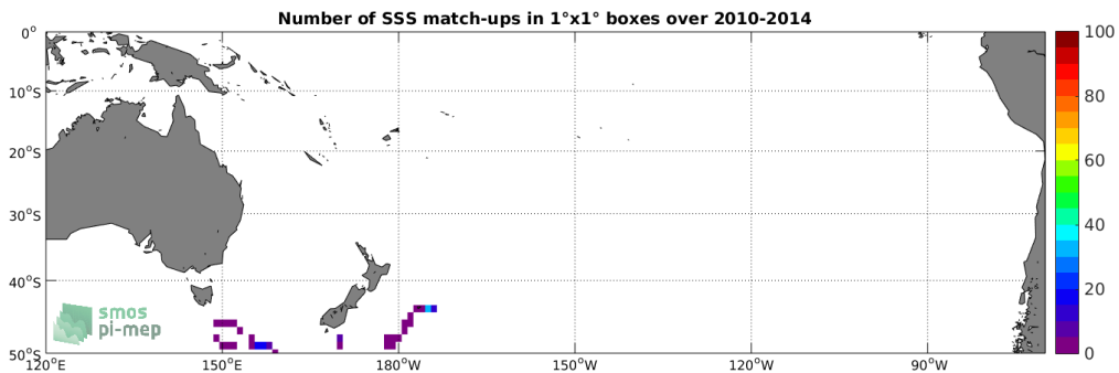
Figure 4: Number of SSS match-ups between Sea mammals SSS and the SMOS-L2-DPGS-v662 SSS product for the South Pacific Ocean Pi-MEP region over 1^\circ \times 1^\circ boxes and for the full satellite product period.
