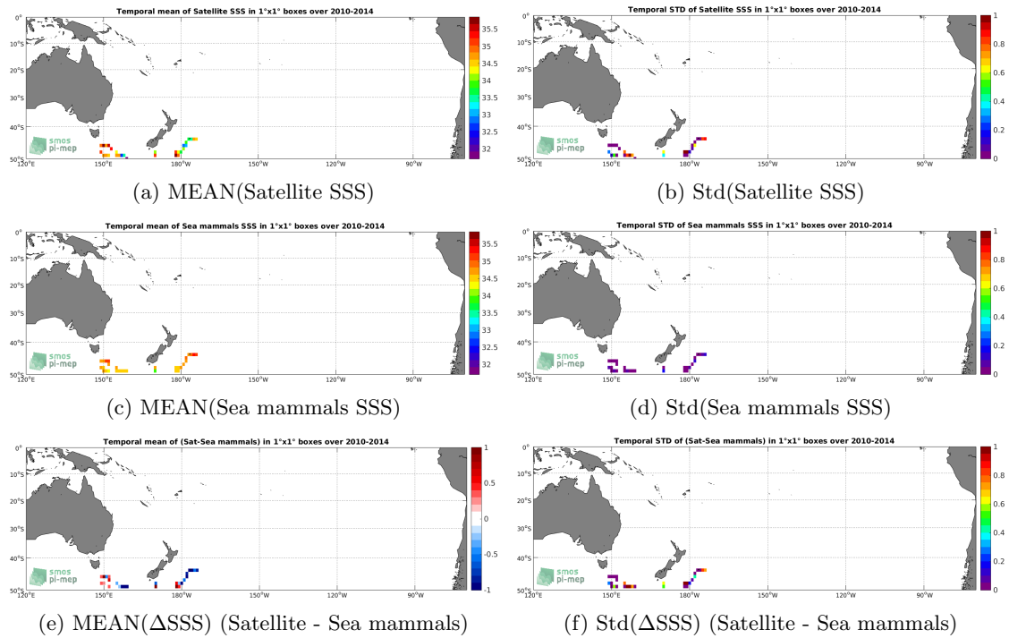
Figure 6: Temporal mean (left) and Std (right) of SSS from SMOS-L2-DPGS-v662 (top), Sea mammals (middle), and of \Delta SSS (Satellite - Sea mammals). Only match-up pairs are used to generate these maps.
