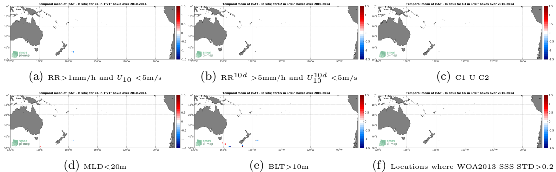
Figure 12: Temporal mean gridded over spatial boxes of size 1^\circ \times 1^\circ of \Delta\text{SSS} (SMOS-L2-DPGS-v662 - Sea mammals) for 6 different subdatasets corresponding to: \text{RR}>1\text{mm/h} and U_{10} <5\text{m/s} (a), \text{RR}^{10d} >5\text{mm/h} and U_{10}^{10d} <5\text{m/s} (b), C1 U C2 (c), \text{MLD}<20\text{m} (d), \text{BLT}>10\text{m} (e), Locations where WOA2013 SSS \text{STD}>0.2 (f).
