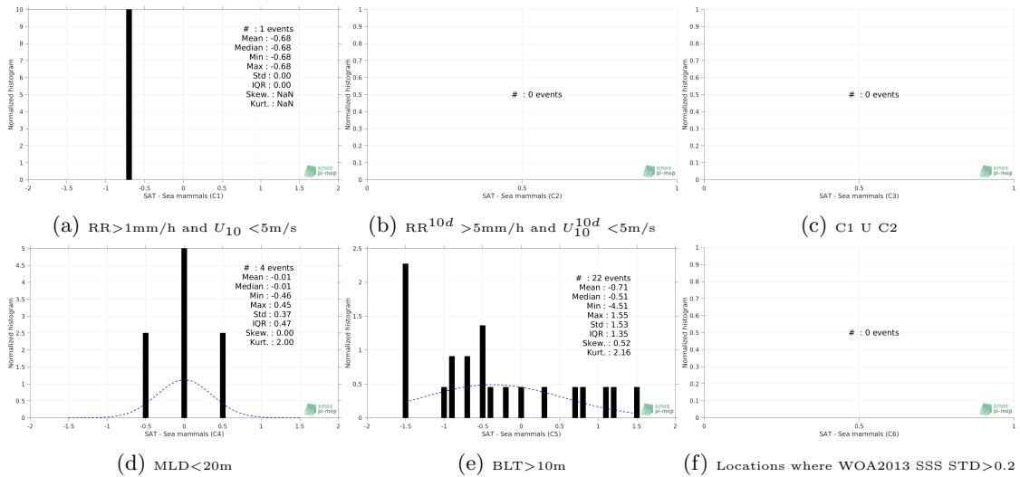
Figure 13: Normalized histogram of \Delta\text{SSS} (SMOS-L2-DPGS-v662 - Sea mammals) for 6 different subdatasets corresponding to: \text{RR}>1\text{mm/h} and U_{10} <5\text{m/s} (a), \text{RR}^{10d} >5\text{mm/h} and U_{10}^{10d} <5\text{m/s} (b), C1 U C2 (c), \text{MLD}<20\text{m} (d), \text{BLT}>10\text{m} (e), Locations where WOA2013 SSS \text{STD}>0.2 (f).
