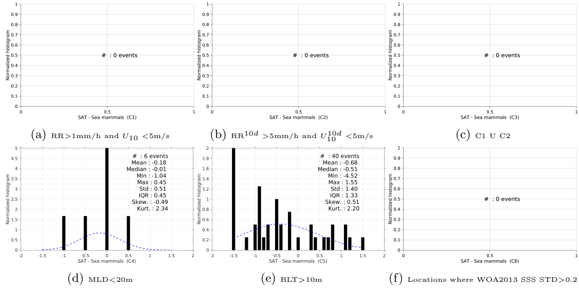
Figure 13: Normalized histogram of \Delta\text{SSS} (SMOS-L2-DPGS-v662 - Sea mammals) for 6 different subdatasets corresponding to: \text{RR} > 1\text{mm/h} and U_{10} < 5\text{m/s} (a), \text{RR}^{10d} > 5\text{mm/h} and U_{10}^{10d} < 5\text{m/s} (b), C1 U C2 (c), \text{MLD} < 20\text{m} (d), \text{BLT} > 10\text{m} (e), Locations where WOA2013 SSS \text{STD} > 0.2 (f).
