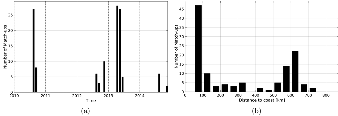
Figure 1: Number of match-ups between Sea mammals and SMOS-L2-DPGS-v662 SSS as a function of time (a) and as function of the distance to coast (b) over the South Pacific Ocean Pi-MEP region and for the full satellite product period.
