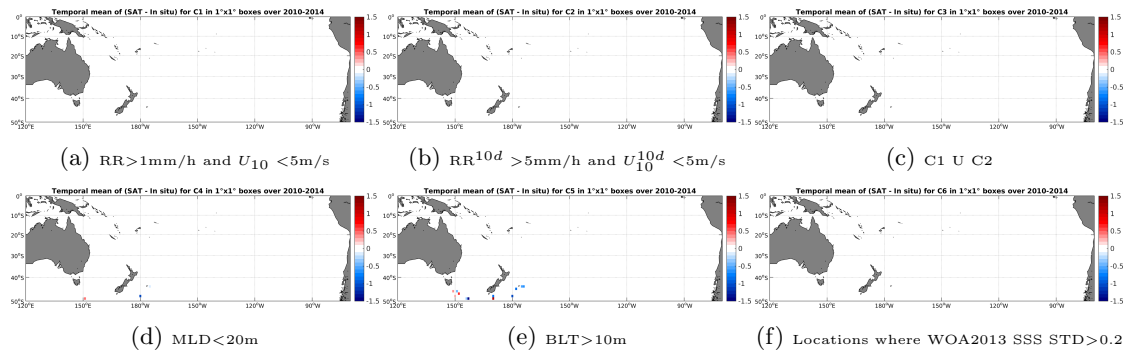
Figure 12: Temporal mean gridded over spatial boxes of size 1^\circ \times 1^\circ of \Delta SSS (SMOS-L2-DPGS-v662 - Sea mammals) for 6 different subdatasets corresponding to: RR > 1\text{mm/h} and U_{10} < 5\text{m/s} (a), RR^{10d} > 5\text{mm/h} and U_{10}^{10d} < 5\text{m/s} (b), C1 U C2 (c), MLD < 20\text{m} (d), BLT > 10\text{m} (e), Locations where WOA2013 SSS STD > 0.2 (f).
