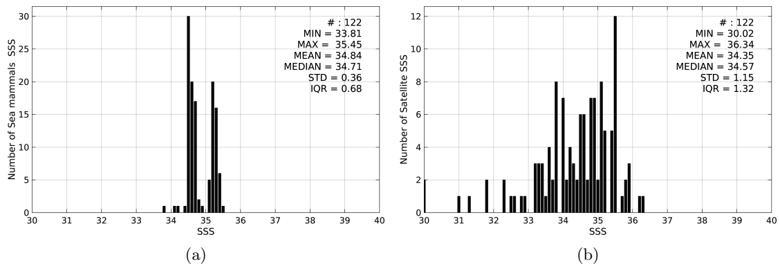
Figure 2: Histograms of SSS from Sea mammals (a) and SMOS-L2-DPGS-v662 (b) considering all match-up pairs per bins of 0.1 over the South Pacific Ocean Pi-MEP region and for the full satellite product period.
