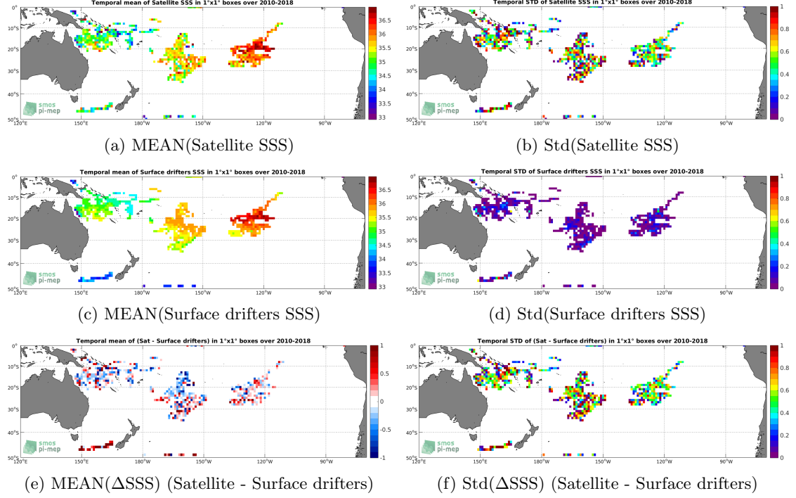
Figure 5: Temporal mean (left) and Std (right) of SSS from SMOS SSS L2 v662 (ESA) (top), Surface drifters (middle), and of \Delta\text{SSS} (Satellite - Surface drifters). Only match-up pairs are used to generate these maps.
