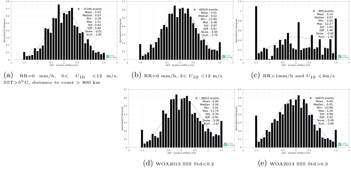
Figure 12: Normalized histogram of \Delta SSS (SMOS SSS L2 v662 (ESA) - Surface drifters) for 5 different subdatasets corresponding to: RR=0 mm/h, 3 < U_{10} < 12 m/s, SST > 5°C, distance to coast > 800 km (a), RR=0 mm/h, 3 < U_{10} < 12 m/s (b), RR > 1mm/h and U_{10} < 4 m/s (c), WOA2013 SSS Std < 0.2 (d), WOA2013 SSS Std > 0.2 (e).
