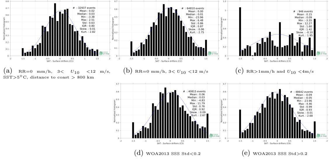
Figure 12: Normalized histogram of \Delta SSS (SMOS SSS L2 v662 (ESA) - Surface drifters) for 5 different subdatasets corresponding to: RR=0 mm/h, 3 < U_{10} < 12 m/s, SST>5°C, distance to coast > 800 km (a), RR=0 mm/h, 3 < U_{10} < 12 m/s (b), RR>1mm/h and U_{10} < 4 m/s (c), WOA2013 SSS Std<0.2 (d), WOA2013 SSS Std>0.2 (e).
