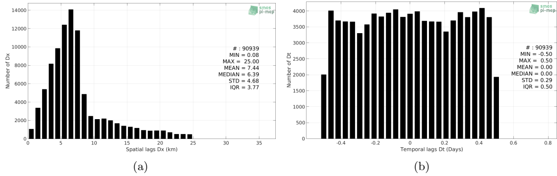
Figure 4: Histograms of the spatial (a) and temporal (b) lags between the time of the Surface drifters measurements and the date of the corresponding SMOS SSS L2 v662 (ESA) SSS product.
