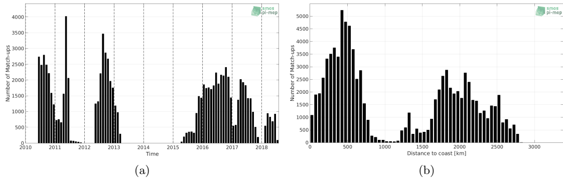
Figure 1: Number of match-ups between Surface drifters and SMOS SSS L2 v662 (ESA) SSS as a function of time (a) and as function of the distance to coast (b) over the South Pacific Ocean Pi-MEP region and for the full satellite product period.
