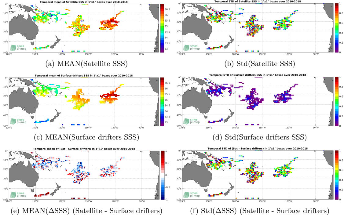
Figure 5: Temporal mean (left) and Std (right) of SSS from SMOS SSS L2 v662 (ESA) (top), Surface drifters (middle), and of \Delta SSS (Satellite - Surface drifters). Only match-up pairs are used to generate these maps.
