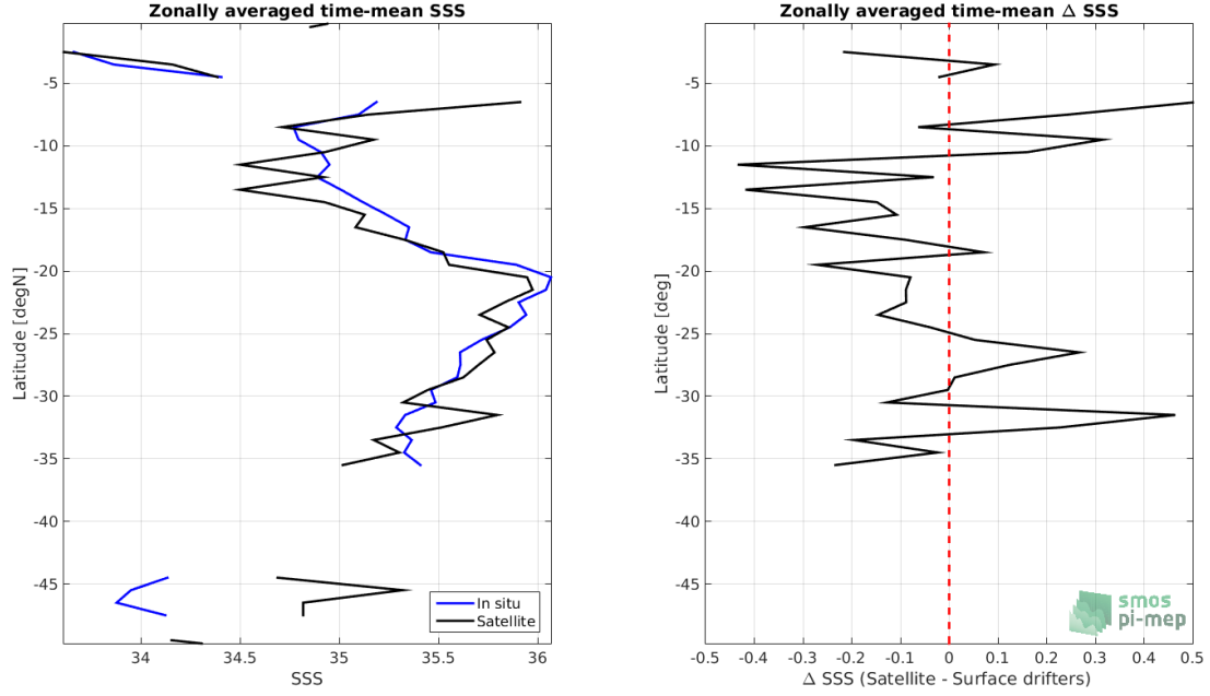
Figure 7: Left panel: Zonal mean SSS from SMOS SSS L2 v662 (ESA) satellite product (black) and from Surface drifters (blue). Right panel: Zonal mean of \Delta SSS (Satellite - Surface drifters) for all the collected Pi-MEP match-up pairs estimated over the full satellite product period.
