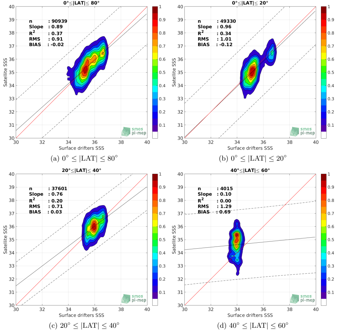
Figure 8: Contour maps of the concentration of SMOS SSS L2 v662 (ESA) SSS (y-axis) versus Surface drifters SSS (x-axis) at match-up pairs for different latitude bands. For each plot, the red line shows x=y . The black thin and dashed lines indicate a linear fit through the data cloud and the \pm 95\% confidence levels, respectively. The number match-up pairs n , the slope and R^2 coefficient of the linear fit, the root mean square (RMS) and the mean bias between satellite and in situ data are indicated for each latitude band in each plots.
