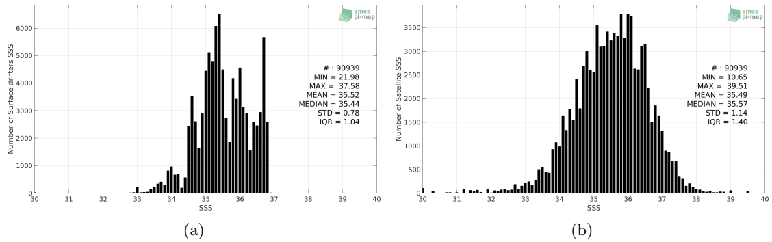
Figure 2: Histograms of SSS from Surface drifters (a) and SMOS SSS L2 v662 (ESA) (b) considering all match-up pairs per bins of 0.1 over the South Pacific Ocean Pi-MEP region and for the full satellite product period.
