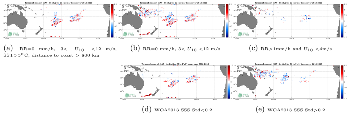
Figure 11: Temporal mean gridded over spatial boxes of size 1^\circ \times 1^\circ of \Delta SSS (SMOS SSS L2 v662 (ESA) - Surface drifters) for 5 different subdatasets corresponding to: RR=0 mm/h, 3 < U_{10} < 12 m/s, SST >5^\circ C, distance to coast > 800 km (a), RR=0 mm/h, 3 < U_{10} < 12 m/s (b), RR>1 mm/h and U_{10} < 4 m/s (c), WOA2013 SSS Std <0.2 (d), WOA2013 SSS Std >0.2 (e).
