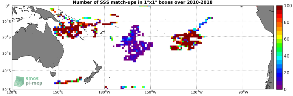
Figure 3: Number of SSS match-ups between Surface drifters SSS and the SMOS SSS L2 v662 (ESA) SSS product for the South Pacific Ocean Pi-MEP region over 1^\circ \times 1^\circ boxes and for the full satellite product period.
