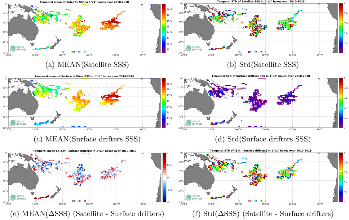
Figure 5: Temporal mean (left) and Std (right) of SSS from SMOS L2 v662 (ESA) (top), Surface drifters (middle), and of \Delta SSS (Satellite - Surface drifters). Only match-up pairs are used to generate these maps.
