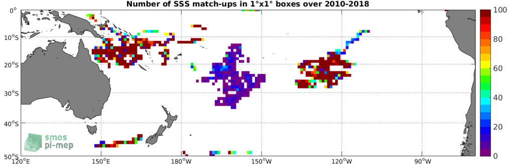
Figure 3: Number of SSS match-ups between Surface drifters SSS and the SMOS L2 v662 (ESA) SSS product for the South Pacific Ocean Pi-MEP region over 1°x1° boxes and for the full satellite product period.
