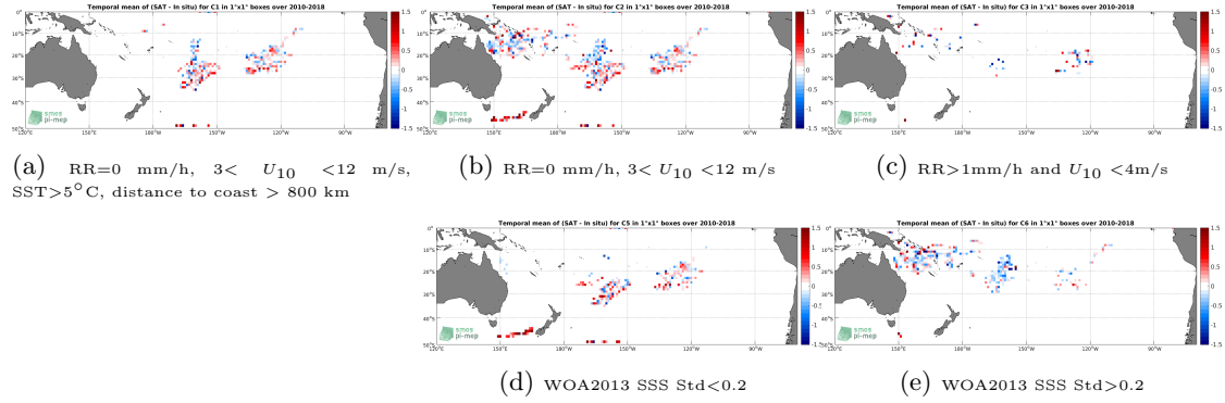
Figure 11: Temporal mean gridded over spatial boxes of size 1^\circ \times 1^\circ of \Delta SSS (SMOS L2 v662 (ESA) - Surface drifters) for 5 different subdatasets corresponding to: RR=0 mm/h, 3 < U_{10} < 12 m/s, SST > 5^\circ\text{C} , distance to coast > 800 km (a), RR=0 mm/h, 3 < U_{10} < 12 m/s (b), RR > 1 mm/h and U_{10} < 4 m/s (c), WOA2013 SSS Std < 0.2 (d), WOA2013 SSS Std > 0.2 (e).
