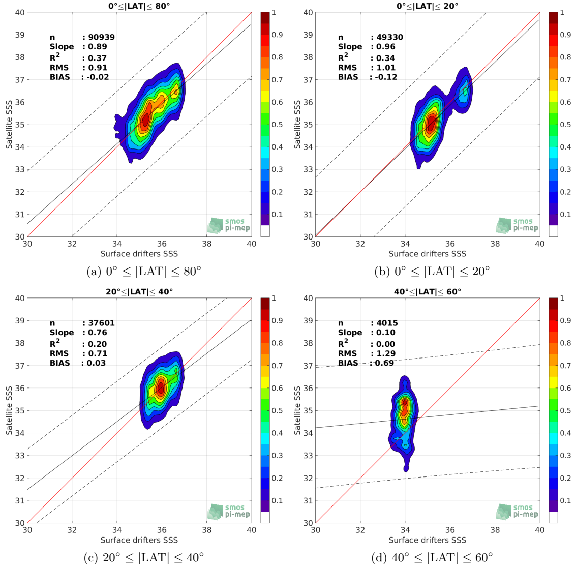
Figure 8: Contour maps of the concentration of SMOS L2 v662 (ESA) SSS (y-axis) versus Surface drifters SSS (x-axis) at match-up pairs for different latitude bands. For each plot, the red line shows x=y . The black thin and dashed lines indicate a linear fit through the data cloud and the \pm 95\% confidence levels, respectively. The number match-up pairs n , the slope and R^2 coefficient of the linear fit, the root mean square (RMS) and the mean bias between satellite and in situ data are indicated for each latitude band in each plots.
