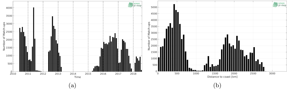
Figure 1: Number of match-ups between Surface drifters and SMOS L2 v662 (ESA) SSS as a function of time (a) and as function of the distance to coast (b) over the South Pacific Ocean Pi-MEP region and for the full satellite product period.
