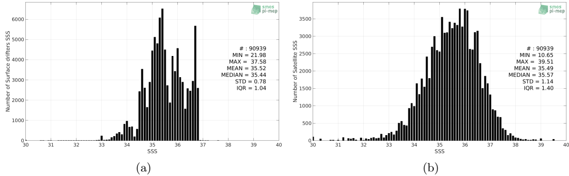
Figure 2: Histograms of SSS from Surface drifters (a) and SMOS L2 v662 (ESA) (b) considering all match-up pairs per bins of 0.1 over the South Pacific Ocean Pi-MEP region and for the full satellite product period.
