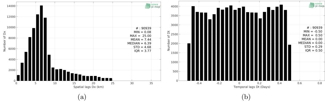
Figure 4: Histograms of the spatial (a) and temporal (b) lags between the time of the Surface drifters measurements and the date of the corresponding SMOS L2 v662 (ESA) SSS product.
