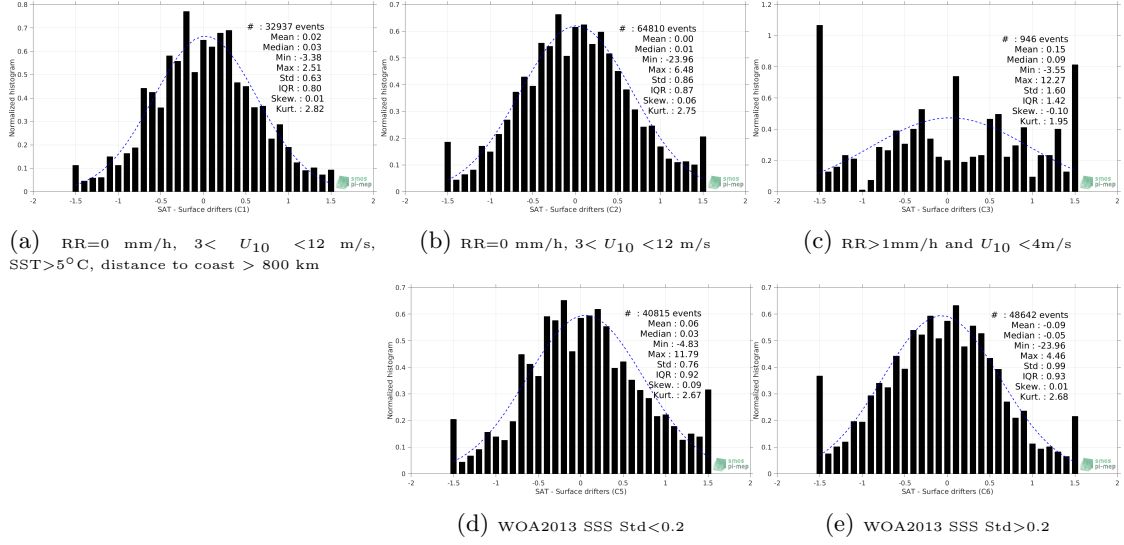
Figure 12: Normalized histogram of \Delta SSS (SMOS L2 v662 (ESA) - Surface drifters) for 5 different subdatasets corresponding to: RR=0 mm/h, 3 < U_{10} < 12 m/s, SST > 5°C, distance to coast > 800 km (a), RR=0 mm/h, 3 < U_{10} < 12 m/s (b), RR > 1mm/h and U_{10} < 4 m/s (c), WOA2013 SSS Std < 0.2 (d), WOA2013 SSS Std > 0.2 (e).
