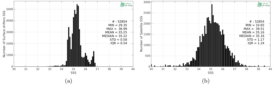
Figure 2: Histograms of SSS from Surface drifters (a) and SMOS-L2-DPGS-v662 (b) considering all match-up pairs per bins of 0.1 over the South Pacific Ocean Pi-MEP region and for the full satellite product period.
