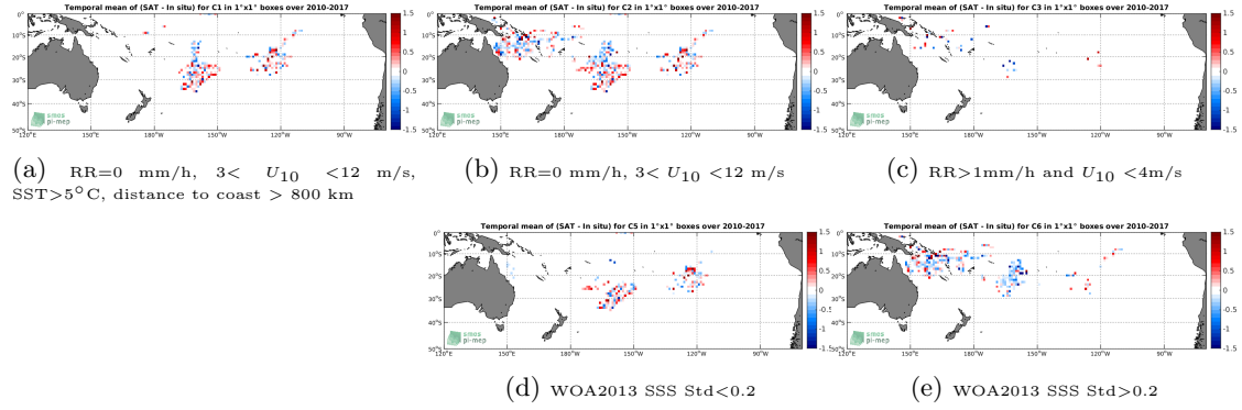
Figure 11: Temporal mean gridded over spatial boxes of size 1^\circ \times 1^\circ of \Delta SSS (SMOS-L2-DPGS-v662 - Surface drifters) for 5 different subdatasets corresponding to: RR=0 mm/h, 3 < U_{10} < 12 m/s, SST > 5^\circ C , distance to coast > 800 km (a), RR=0 mm/h, 3 < U_{10} < 12 m/s (b), RR > 1 mm/h and U_{10} < 4 m/s (c), WOA2013 SSS Std < 0.2 (d), WOA2013 SSS Std > 0.2 (e).
