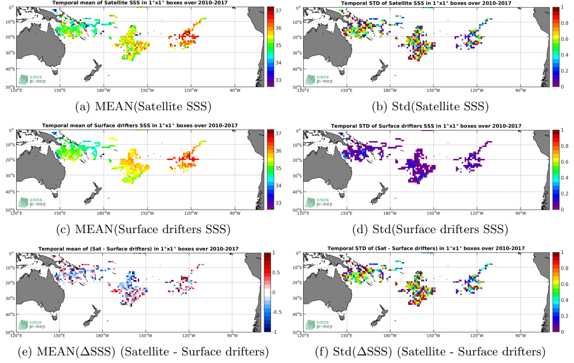
Figure 5: Temporal mean (left) and Std (right) of SSS from SMOS-L2-DPGS-v662 (top), Surface drifters (middle), and of \Delta SSS (Satellite - Surface drifters). Only match-up pairs are used to generate these maps.
