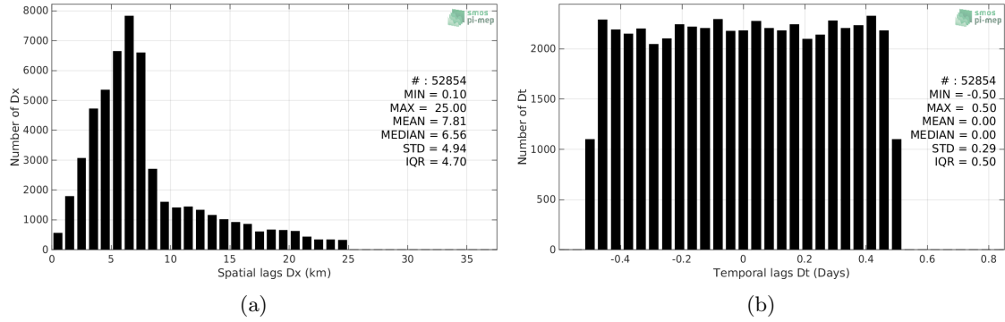
Figure 4: Histograms of the spatial (a) and temporal (b) lags between the time of the Surface drifters measurements and the date of the corresponding SMOS-L2-DPGS-v662 SSS product.
