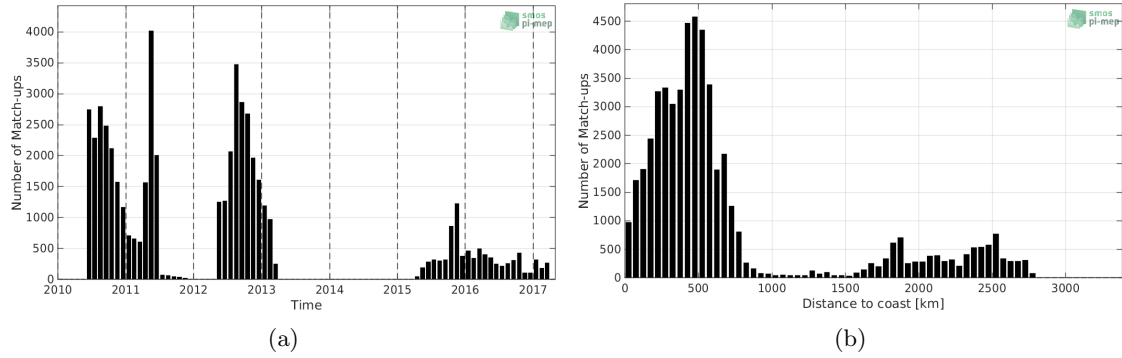
Figure 1: Number of match-ups between Surface drifters and SMOS-L2-DPGS-v662 SSS as a function of time (a) and as function of the distance to coast (b) over the South Pacific Ocean Pi-MEP region and for the full satellite product period.
