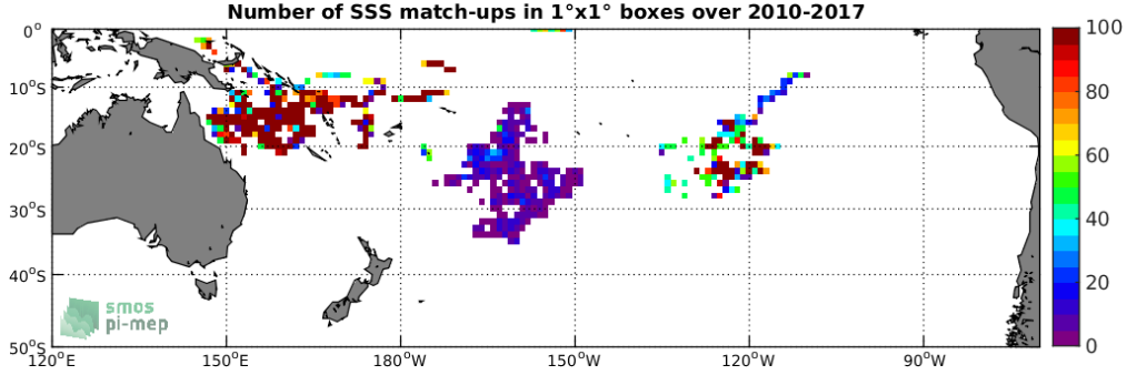
Figure 3: Number of SSS match-ups between Surface drifters SSS and the SMOS-L2-DPGS-v662 SSS product for the South Pacific Ocean Pi-MEP region over 1^\circ \times 1^\circ boxes and for the full satellite product period.
