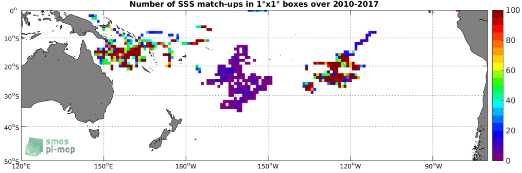
Figure 3: Number of SSS match-ups between Surface drifters SSS and the SMOS-L2-DPGS-v662 SSS product for the South Pacific Ocean Pi-MEP region over 1°x1° boxes and for the full satellite product period.
