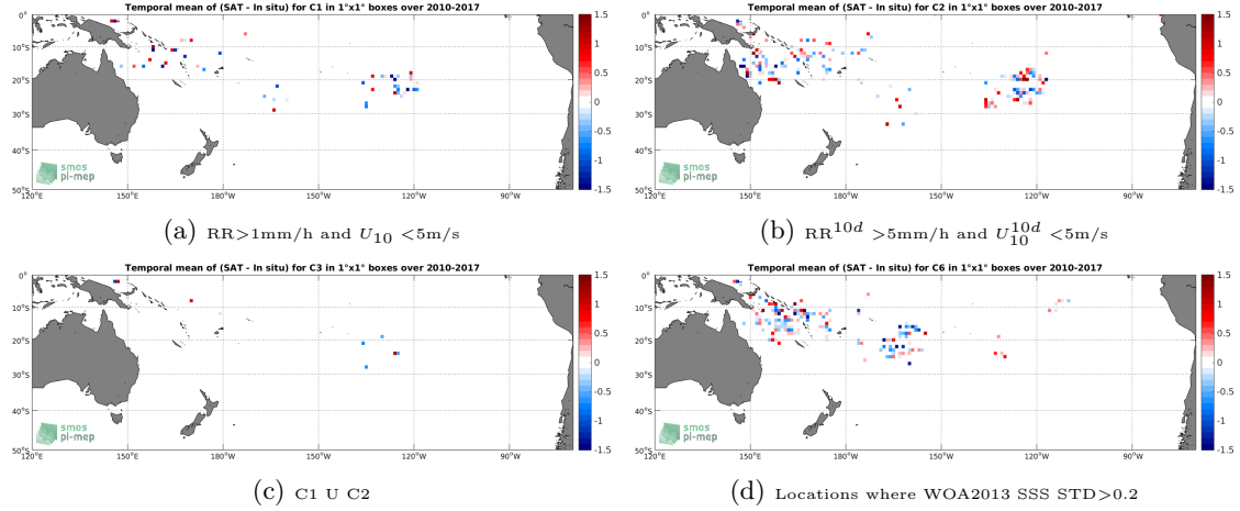
Figure 11: Temporal mean gridded over spatial boxes of size 1^\circ \times 1^\circ of \Delta SSS (SMOS-L2-DPGS-v662 - Surface drifters) for 4 different subdatasets corresponding to: RR > 1\text{mm/h} and U_{10} < 5\text{m/s} (a), RR^{10d} > 5\text{mm/h} and U_{10}^{10d} < 5\text{m/s} (b), C1 U C2 (c), Locations where WOA2013 SSS STD > 0.2 (d).
