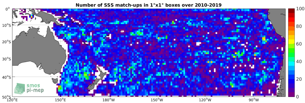
Figure 4: Number of SSS match-ups between Argos SSS and the SMOS-L2-DPGS-v662 SSS product for the South Pacific Ocean Pi-MEP region over 1^\circ \times 1^\circ boxes and for the full satellite product period.
