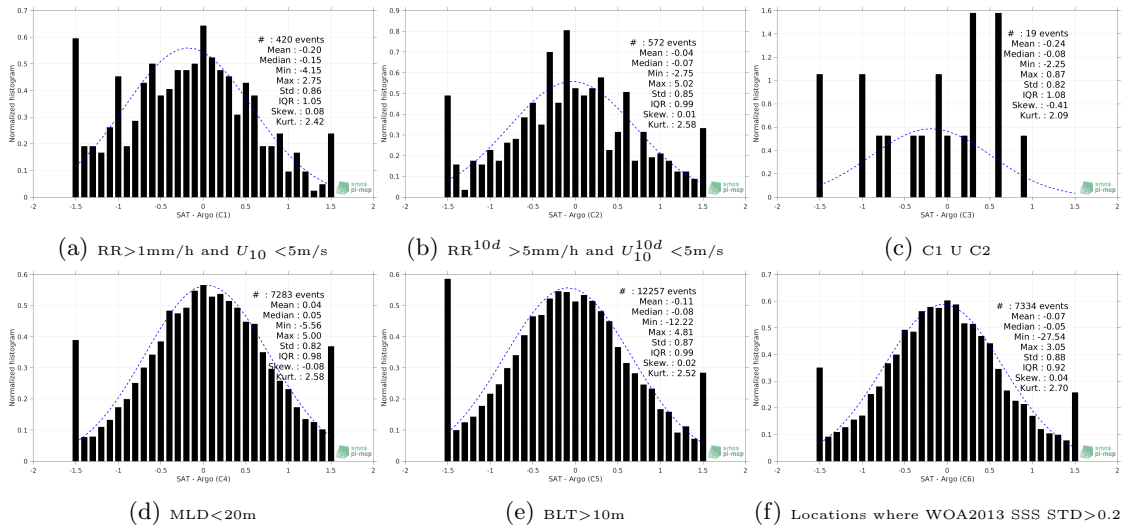
Figure 13: Normalized histogram of \Delta SSS (SMOS-L2-DPGS-v662 - Argo) for 6 different subdatasets corresponding to: RR>1mm/h and U_{10} <5m/s (a), RR^{10d} >5mm/h and U_{10}^{10d} <5m/s (b), C1 U C2 (c),MLD<20m (d),BLT>10m (e),Locations where WOA2013 SSS STD>0.2 (f).
