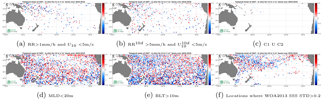
Figure 12: Temporal mean gridded over spatial boxes of size 1°x1° of \Delta SSS (SMOS-L2-DPGS-v662 - Argo) for 6 different subdatasets corresponding to:RR>1mm/h and U_{10} <5m/s (a), RR^{10d} >5mm/h and U_{10}^{10d} <5m/s (b), C1 U C2 (c),MLD<20m (d),BLT>10m (e),Locations where WOA2013 SSS STD>0.2 (f).
