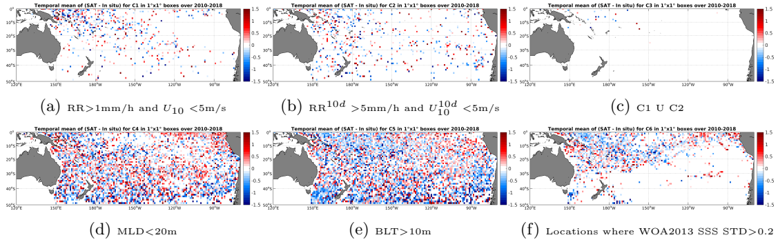
Figure 12: Temporal mean gridded over spatial boxes of size 1^\circ \times 1^\circ of \Delta SSS (SMOS-L2-DPGS-v662 - Argo) for 6 different subdatasets corresponding to: RR > 1\text{mm/h} and U_{10} < 5\text{m/s} (a), RR^{10d} > 5\text{mm/h} and U_{10}^{10d} < 5\text{m/s} (b), C1 U C2 (c), MLD < 20\text{m} (d), BLT > 10\text{m} (e), Locations where WOA2013 SSS STD > 0.2 (f).
