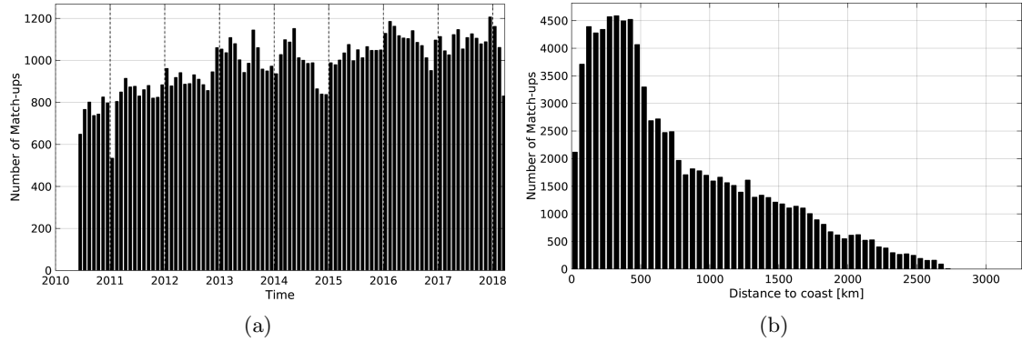
Figure 1: Number of match-ups between Argo and SMOS-L2-DPGS-v662 SSS as a function of time (a) and as function of the distance to coast (b) over the South Pacific Ocean Pi-MEP region and for the full satellite product period.
