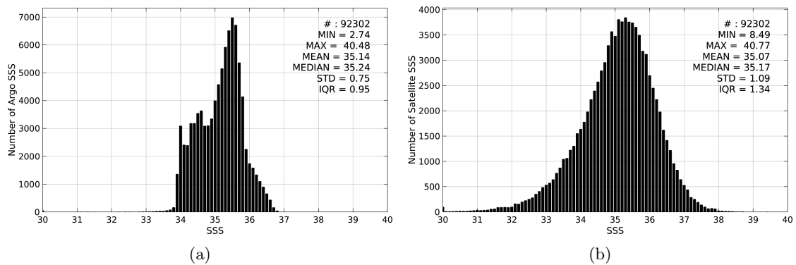
Figure 2: Histograms of SSS from Argo (a) and SMOS-L2-DPGS-v662 (b) considering all match-up pairs per bins of 0.1 over the South Pacific Ocean Pi-MEP region and for the full satellite product period.
