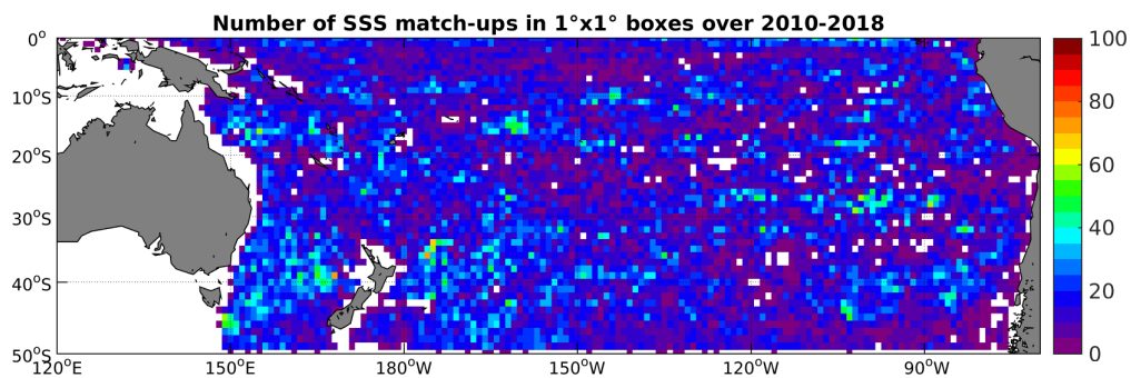
Figure 4: Number of SSS match-ups between Argon SSS and the SMOS-L2-DPGS-v662 SSS product for the South Pacific Ocean Pi-MEP region over 1°x1° boxes and for the full satellite product period.
