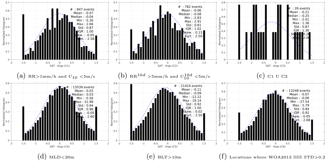
Figure 13: Normalized histogram of \Delta SSS (SMOS-L2-DPGS-v662 - Argo) for 6 different subdatasets corresponding to: RR > 1\text{mm/h} and U_{10} < 5\text{m/s} (a), RR^{10d} > 5\text{mm/h} and U_{10}^{10d} < 5\text{m/s} (b), C1 U C2 (c), MLD < 20\text{m} (d), BLT > 10\text{m} (e), Locations where WOA2013 SSS STD > 0.2 (f).
