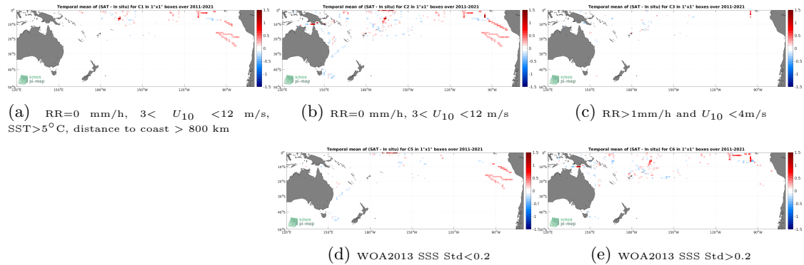
Figure 12: Temporal mean gridded over spatial boxes of size 1^\circ \times 1^\circ of \Delta SSS (SMAP SSS L4 OI v1 - 7 Days (IPRC) - TSG (SAMOS)) for 5 different subdatasets corresponding to:RR=0 mm/h, 3 < U_{10} < 12 m/s, SST >5^\circ\text{C} , distance to coast > 800 km (a), RR=0 mm/h, 3 < U_{10} < 12 m/s (b), RR >1 mm/h and U_{10} < 4 m/s (c), WOA2013 SSS Std <0.2 (d), WOA2013 SSS Std >0.2 (e).
