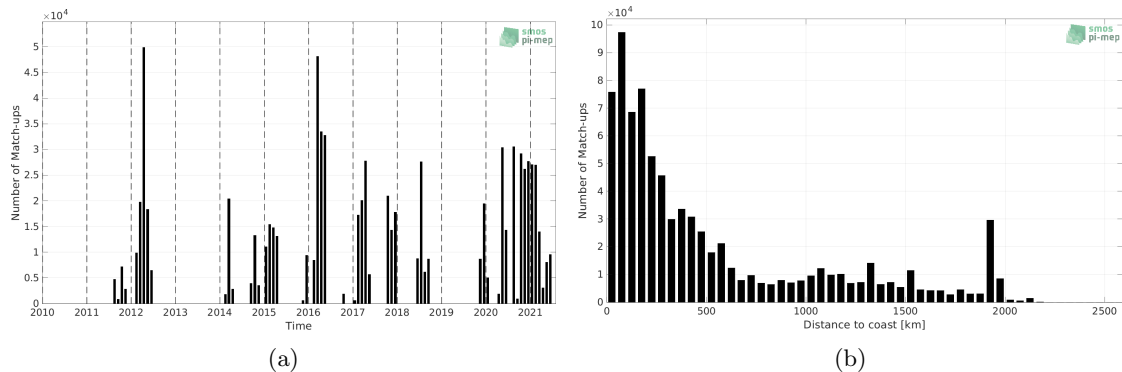
Figure 1: Number of match-ups between TSG (SAMOS) and SMAP SSS L4 OI v1 - 7 Days (IPRC) SSS as a function of time (a) and as function of the distance to coast (b) over the South Pacific Ocean Pi-MEP region and for the full satellite product period.
