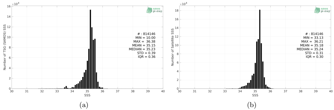
Figure 2: Histograms of SSS from TSG (SAMOS) (a) and SMAP SSS L4 OI v1 - 7 Days (IPRC) (b) considering all match-up pairs per bins of 0.1 over the South Pacific Ocean Pi-MEP region and for the full satellite product period.
