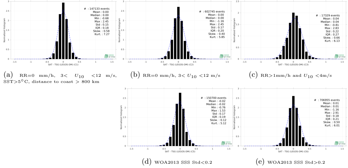
Figure 13: Normalized histogram of \Delta SSS (SMAP SSS L4 OI v1 - 7 Days (IPRC) - TSG (LEGOS-DM)) for 5 different subdatasets corresponding to: RR=0 mm/h, 3 < U_{10} < 12 m/s, SST > 5°C, distance to coast > 800 km (a), RR=0 mm/h, 3 < U_{10} < 12 m/s (b), RR > 1mm/h and U_{10} < 4 m/s (c), WOA2013 SSS Std < 0.2 (d), WOA2013 SSS Std > 0.2 (e).
