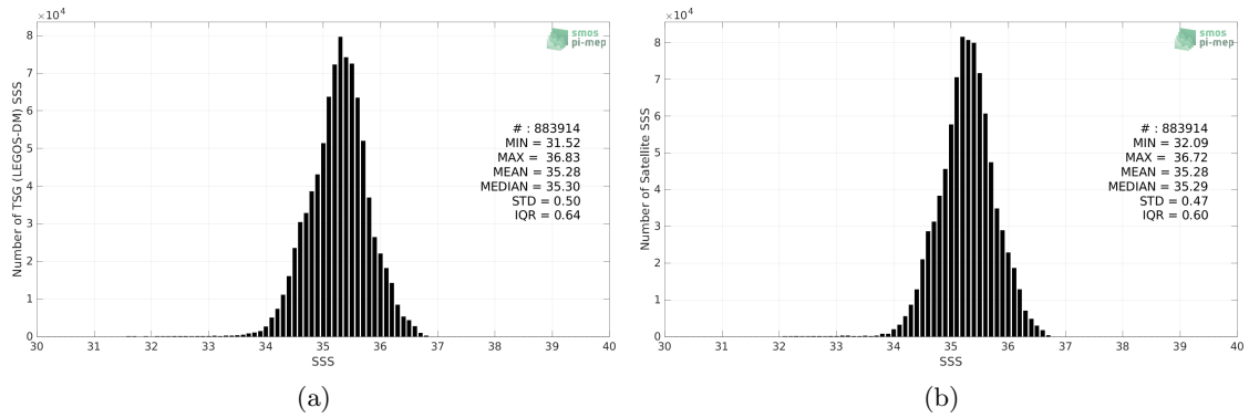
Figure 2: Histograms of SSS from TSG (LEGOS-DM) (a) and SMAP SSS L4 OI v1 - 7 Days (IPRC) (b) considering all match-up pairs per bins of 0.1 over the South Pacific Ocean Pi-MEP region and for the full satellite product period.
