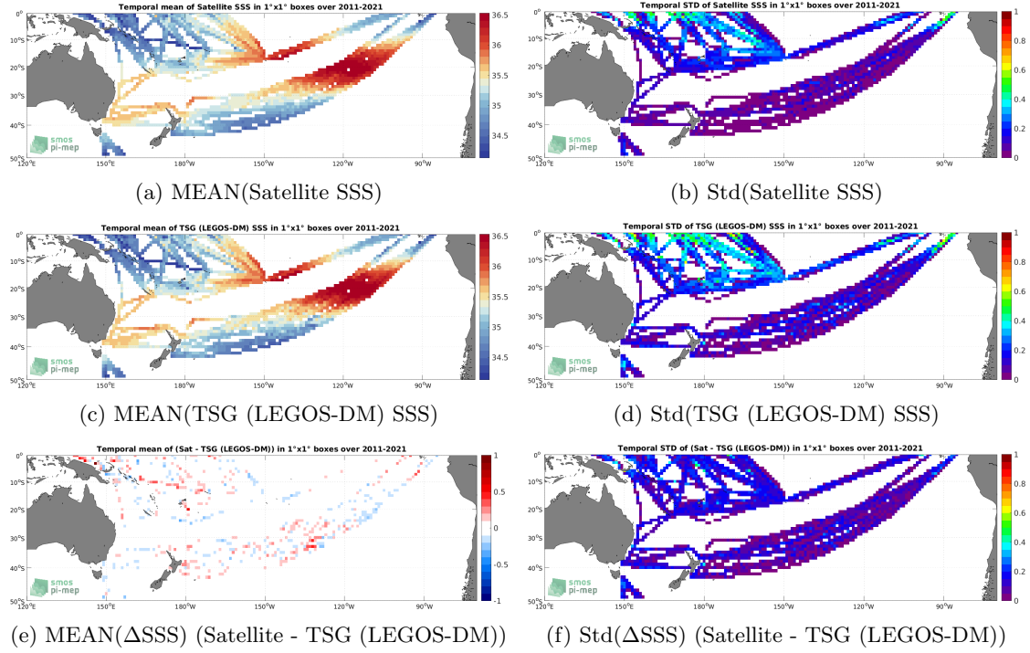
Figure 6: Temporal mean (left) and Std (right) of SSS from SMAP SSS L4 OI v1 - 7 Days (IPRC) (top), TSG (LEGOS-DM) (middle), and of \Delta SSS (Satellite - TSG (LEGOS-DM)). Only match-up pairs are used to generate these maps.
