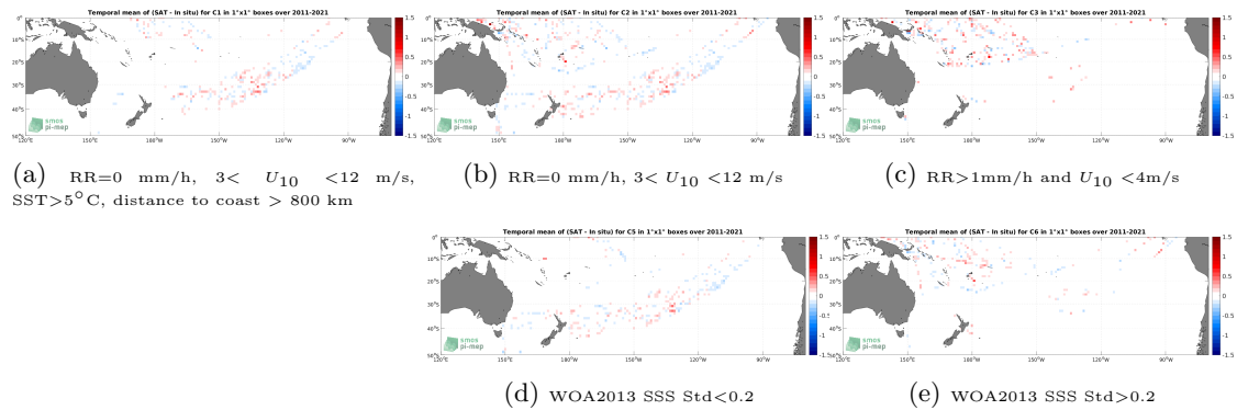
Figure 12: Temporal mean gridded over spatial boxes of size 1^\circ \times 1^\circ of \Delta SSS (SMAP SSS L4 OI v1 - 7 Days (IPRC) - TSG (LEGOS-DM)) for 5 different subdatasets corresponding to:RR=0 mm/h, 3 < U_{10} < 12 m/s, SST >5^\circ C, distance to coast > 800 km (a), RR=0 mm/h, 3 < U_{10} < 12 m/s (b), RR >1 mm/h and U_{10} < 4 m/s (c), WOA2013 SSS Std <0.2 (d), WOA2013 SSS Std >0.2 (e).
