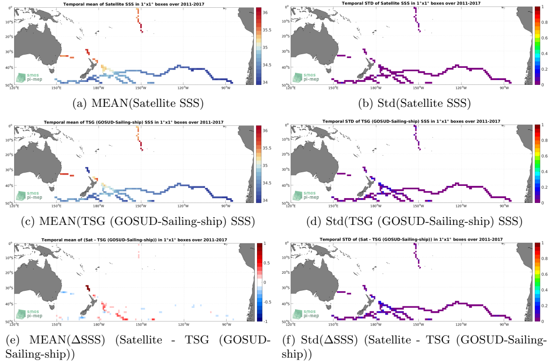
Figure 6: Temporal mean (left) and Std (right) of SSS from SMAP SSS L4 OI v1 - 7 Days (IPRC) (top), TSG (GOSUD-Sailing-ship) (middle), and of \Delta SSS (Satellite - TSG (GOSUD-Sailing-ship)). Only match-up pairs are used to generate these maps.
