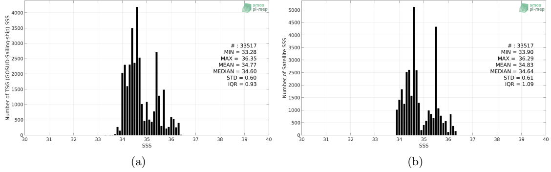
Figure 2: Histograms of SSS from TSG (GOSUD-Sailing-ship) (a) and SMAP SSS L4 OI v1 - 7 Days (IPRC) (b) considering all match-up pairs per bins of 0.1 over the South Pacific Ocean Pi-MEP region and for the full satellite product period.
