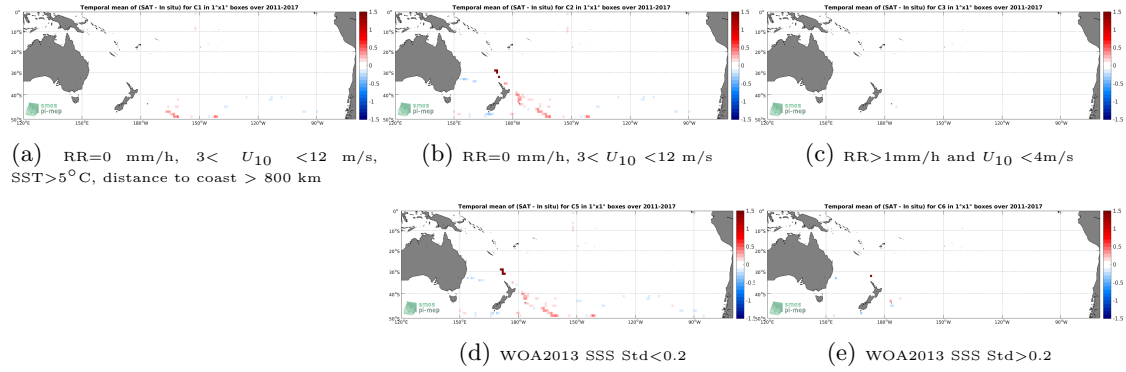
Figure 12: Temporal mean gridded over spatial boxes of size 1^\circ \times 1^\circ of \Delta SSS (SMAP SSS L4 OI v1 - 7 Days (IPRC) - TSG (GOSUD-Sailing-ship)) for 5 different subdatasets corresponding to: RR=0 mm/h, 3 < U_{10} < 12 m/s, SST >5^\circ\text{C} , distance to coast > 800 km (a), RR=0 mm/h, 3 < U_{10} < 12 m/s (b), RR>1\text{mm/h} and U_{10} < 4\text{m/s} (c), WOA2013 SSS Std <0.2 (d), WOA2013 SSS Std >0.2 (e).
