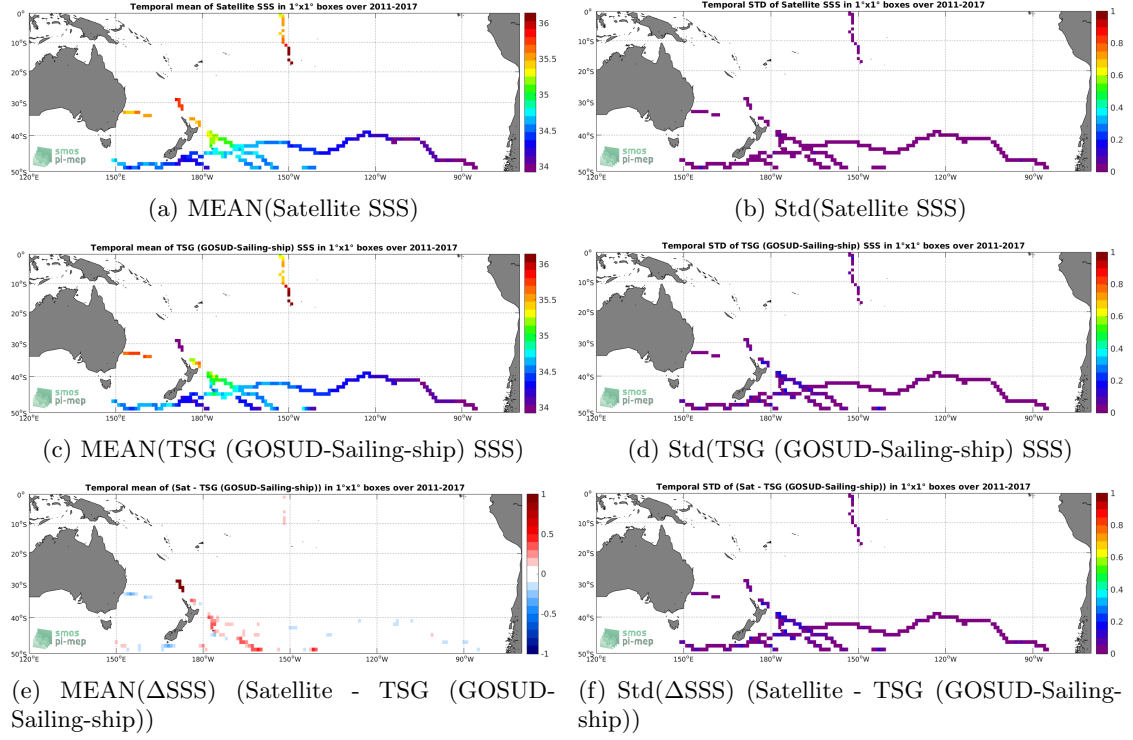
Figure 6: Temporal mean (left) and Std (right) of SSS from SMAP SSS L4 OI v1 - 7 Days (IPRC) (top), TSG (GOSUD-Sailing-ship) (middle), and of \Delta SSS (Satellite - TSG (GOSUD-Sailing-ship)). Only match-up pairs are used to generate these maps.
