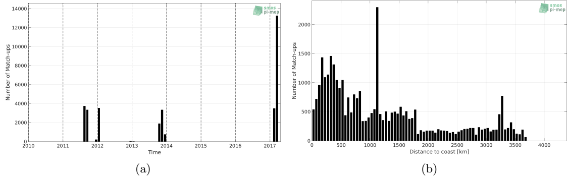
Figure 1: Number of match-ups between TSG (GOSUD-Sailing-ship) and SMAP SSS L4 OI v1 - 7 Days (IPRC) SSS as a function of time (a) and as function of the distance to coast (b) over the South Pacific Ocean Pi-MEP region and for the full satellite product period.
