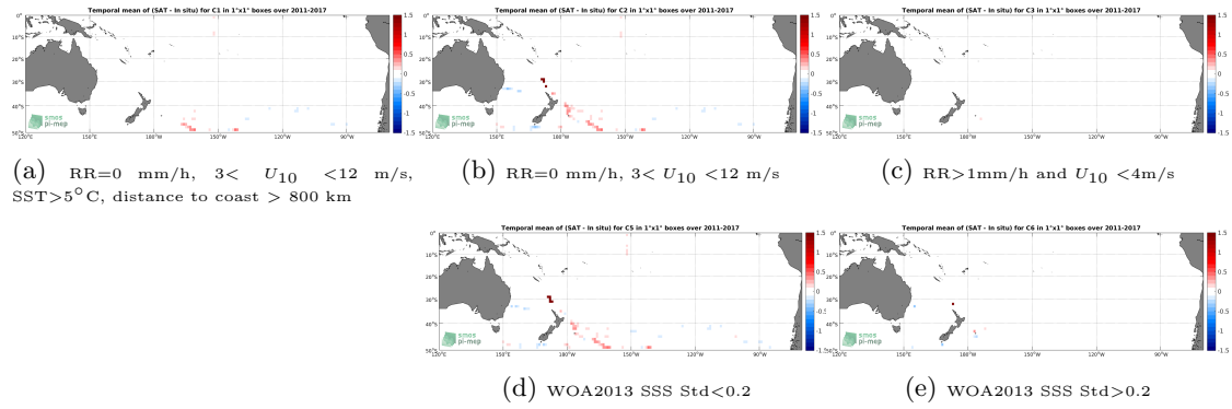
Figure 12: Temporal mean gridded over spatial boxes of size 1^\circ \times 1^\circ of \Delta SSS (SMAP SSS L4 OI v1 - 7day (IPRC) - TSG (GOSUD-Sailing-ship)) for 5 different subdatasets corresponding to: RR=0 mm/h, 3 < U_{10} < 12 m/s, SST >5^\circ\text{C} , distance to coast > 800 km (a), RR=0 mm/h, 3 < U_{10} < 12 m/s (b), RR>1\text{mm/h} and U_{10} < 4\text{m/s} (c), WOA2013 SSS Std <0.2 (d), WOA2013 SSS Std >0.2 (e).
