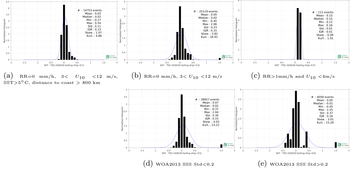
Figure 13: Normalized histogram of \Delta SSS (SMAP SSS L4 OI v1 - 7day (IPRC) - TSG (GOSUD-Sailing-ship)) for 5 different subdatasets corresponding to: RR=0 mm/h, 3 < U_{10} < 12 m/s, SST>5°C, distance to coast > 800 km (a), RR=0 mm/h, 3 < U_{10} < 12 m/s (b), RR>1 mm/h and U_{10} < 4 m/s (c), WOA2013 SSS Std<0.2 (d), WOA2013 SSS Std>0.2 (e).
