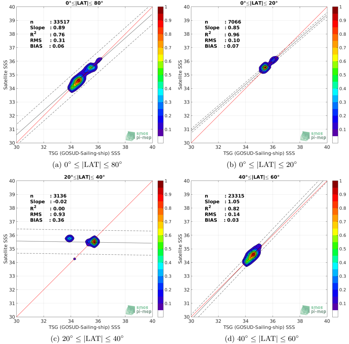
Figure 9: Contour maps of the concentration of SMAP SSS L4 OI v1 - 7day (IPRC) SSS (y-axis) versus TSG (GOSUD-Sailing-ship) SSS (x-axis) at match-up pairs for different latitude bands. For each plot, the red line shows x=y . The black thin and dashed lines indicate a linear fit through the data cloud and the \pm 95\% confidence levels, respectively. The number match-up pairs n , the slope and R^2 coefficient of the linear fit, the root mean square (RMS) and the mean bias between satellite and in situ data are indicated for each latitude band in each plots.
