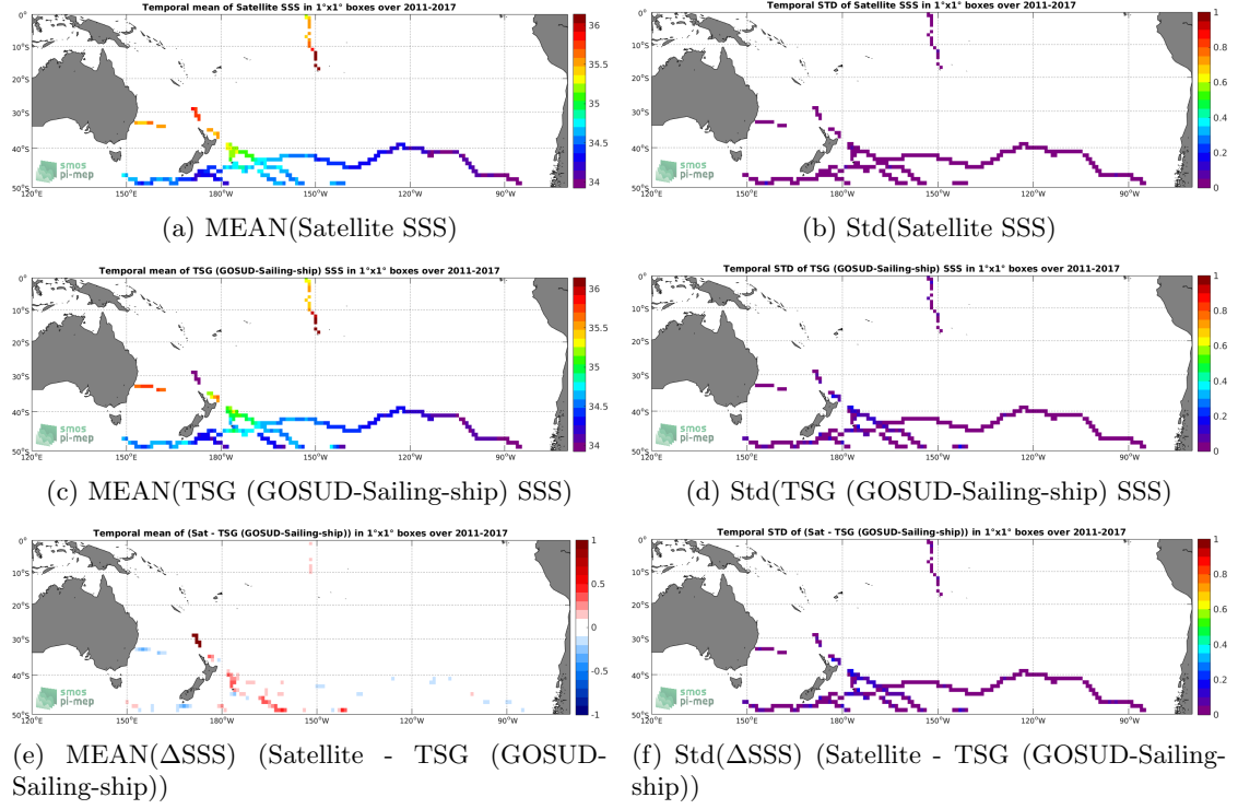
Figure 6: Temporal mean (left) and Std (right) of SSS from SMAP SSS L4 OI v1 - 7day (IPRC) (top), TSG (GOSUD-Sailing-ship) (middle), and of \Delta SSS (Satellite - TSG (GOSUD-Sailing-ship)). Only match-up pairs are used to generate these maps.
