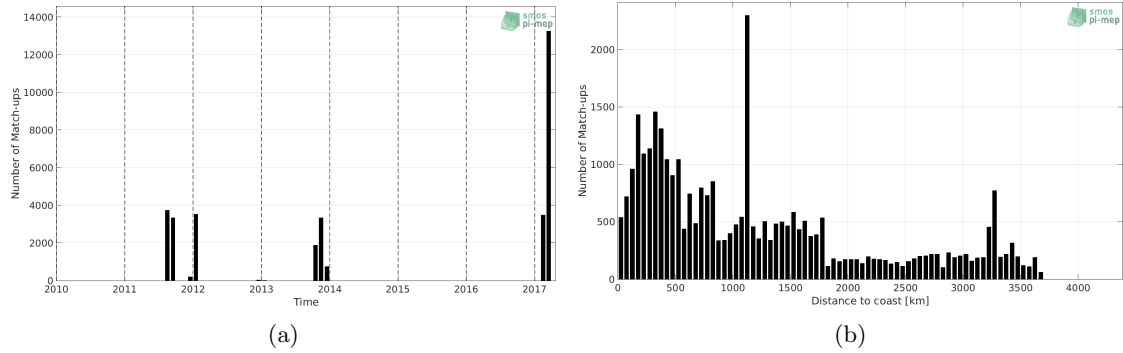
Figure 1: Number of match-ups between TSG (GOSUD-Sailing-ship) and SMAP SSS L4 OI v1 - 7day (IPRC) SSS as a function of time (a) and as function of the distance to coast (b) over the South Pacific Ocean Pi-MEP region and for the full satellite product period.
