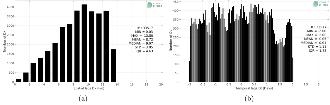
Figure 5: Histograms of the spatial (a) and temporal (b) lags between the location/time of the TSG (GOSUD-Sailing-ship) measurement and the date of the corresponding SMAP SSS L4 OI v1 - 7day (IPRC) SSS pixel.
