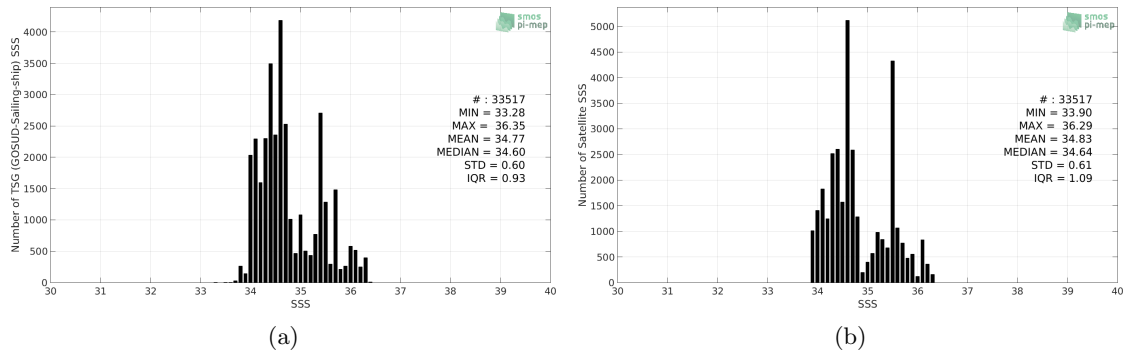
Figure 2: Histograms of SSS from TSG (GOSUD-Sailing-ship) (a) and SMAP SSS L4 OI v1 - 7day (IPRC) (b) considering all match-up pairs per bins of 0.1 over the South Pacific Ocean Pi-MEP region and for the full satellite product period.
