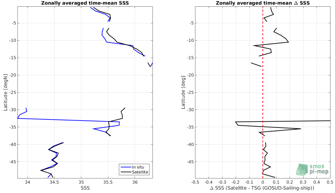
Figure 8: Left panel: Zonal mean SSS from SMAP SSS L4 OI v1 - 7day (IPRC) satellite product (black) and from TSG (GOSUD-Sailing-ship) (blue). Right panel: Zonal mean of \Delta SSS (Satellite - TSG (GOSUD-Sailing-ship)) for all the collected Pi-MEP match-up pairs estimated over the full satellite product period.
