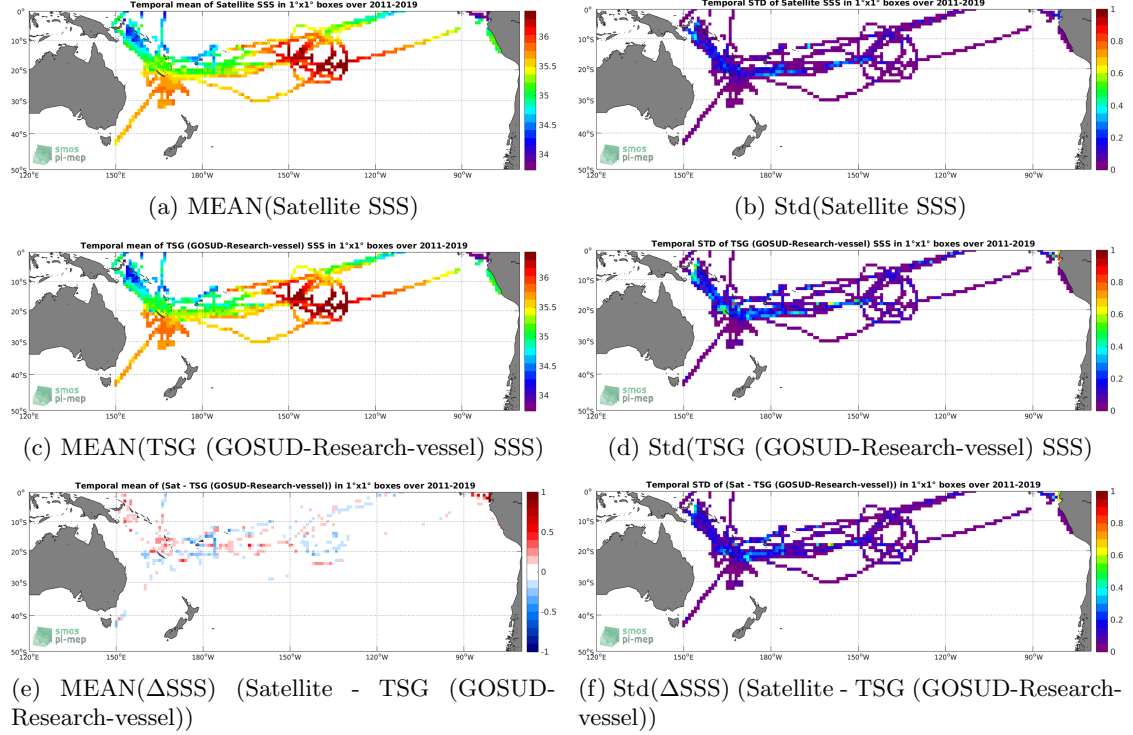
Figure 6: Temporal mean (left) and Std (right) of SSS from SMAP SSS L4 OI v1 - 7 Days (IPRC) (top), TSG (GOSUD-Research-vessel) (middle), and of \Delta SSS (Satellite - TSG (GOSUD-Research-vessel)). Only match-up pairs are used to generate these maps.
