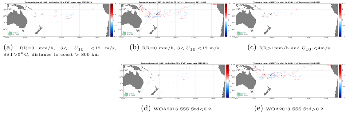
Figure 12: Temporal mean gridded over spatial boxes of size 1^\circ \times 1^\circ of \Delta SSS (SMAP SSS L4 OI v1 - 7day (IPRC) - TSG (GOSUD-Research-vessel)) for 5 different subdatasets corresponding to: RR=0 mm/h, 3 < U_{10} < 12 m/s, SST > 5^\circ\text{C} , distance to coast > 800 km (a), RR=0 mm/h, 3 < U_{10} < 12 m/s (b), RR > 1 mm/h and U_{10} < 4 m/s (c), WOA2013 SSS Std < 0.2 (d), WOA2013 SSS Std > 0.2 (e).
