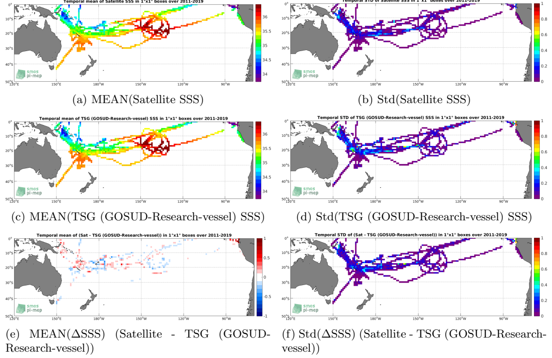
Figure 6: Temporal mean (left) and Std (right) of SSS from SMAP SSS L4 OI v1 - 7day (IPRC) (top), TSG (GOSUD-Research-vessel) (middle), and of \Delta SSS (Satellite - TSG (GOSUD-Research-vessel)). Only match-up pairs are used to generate these maps.
