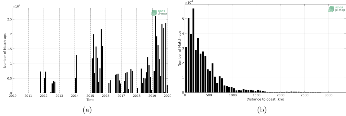
Figure 1: Number of match-ups between TSG (GOSUD-Research-vessel) and SMAP SSS L4 OI v1 - 7day (IPRC) SSS as a function of time (a) and as function of the distance to coast (b) over the South Pacific Ocean Pi-MEP region and for the full satellite product period.
