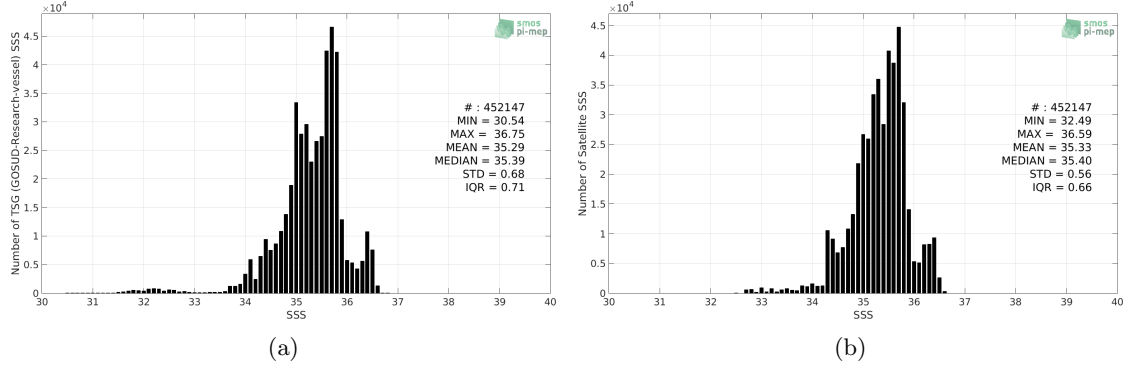
Figure 2: Histograms of SSS from TSG (GOSUD-Research-vessel) (a) and SMAP SSS L4 OI v1 - 7day (IPRC) (b) considering all match-up pairs per bins of 0.1 over the South Pacific Ocean Pi-MEP region and for the full satellite product period.
