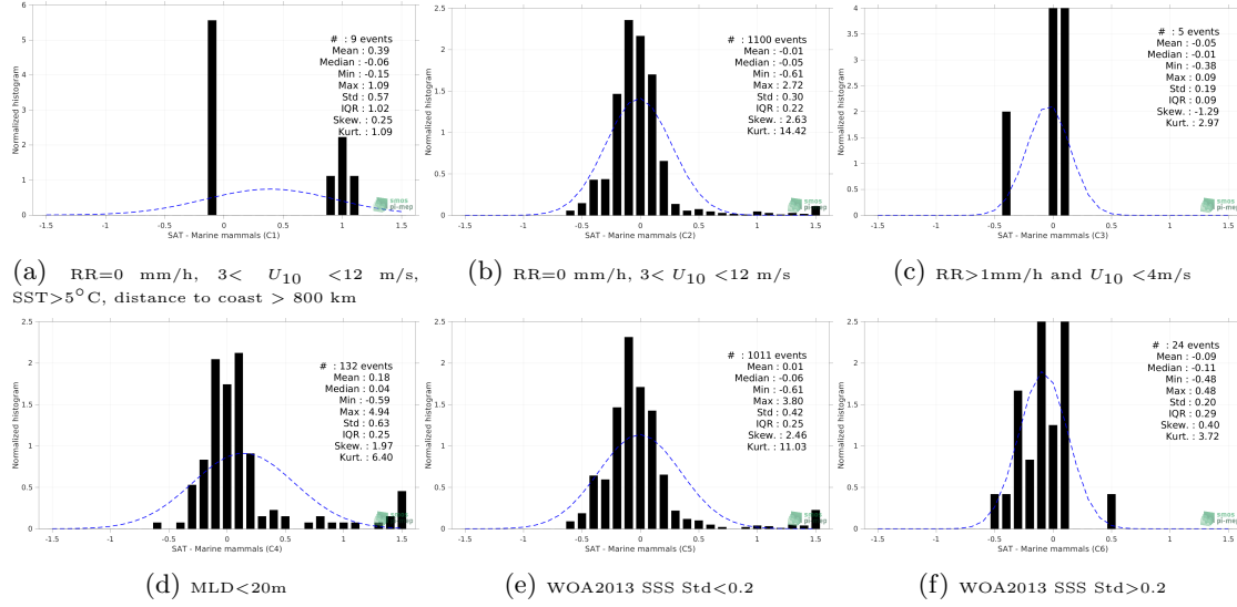
Figure 13: Normalized histogram of \Delta\text{SSS} (SMAP SSS L4 OI v1 - 7 Days (IPRC) - Marine mammals) for 6 different subdatasets corresponding to: RR=0 mm/h, 3 < U_{10} < 12 m/s, SST>5°C, distance to coast > 800 km (a), RR=0 mm/h, 3 < U_{10} < 12 m/s (b), RR>1mm/h and U_{10} < 4 m/s (c), MLD<20m (d), WOA2013 SSS Std<0.2 (e), WOA2013 SSS Std>0.2 (f).
