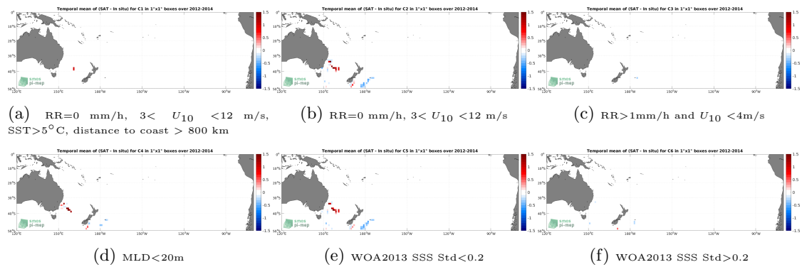
Figure 12: Temporal mean gridded over spatial boxes of size 1^\circ \times 1^\circ of \Delta SSS (SMAP SSS L4 OI v1 - 7 Days (IPRC) - Marine mammals) for 6 different subdatasets corresponding to:RR=0 mm/h, 3 < U_{10} < 12 m/s, SST >5^\circ C, distance to coast > 800 km (a), RR=0 mm/h, 3 < U_{10} < 12 m/s (b), RR >1 mm/h and U_{10} < 4 m/s (c),MLD <20 m (d),WOA2013 SSS Std <0.2 (e),WOA2013 SSS Std >0.2 (f).
