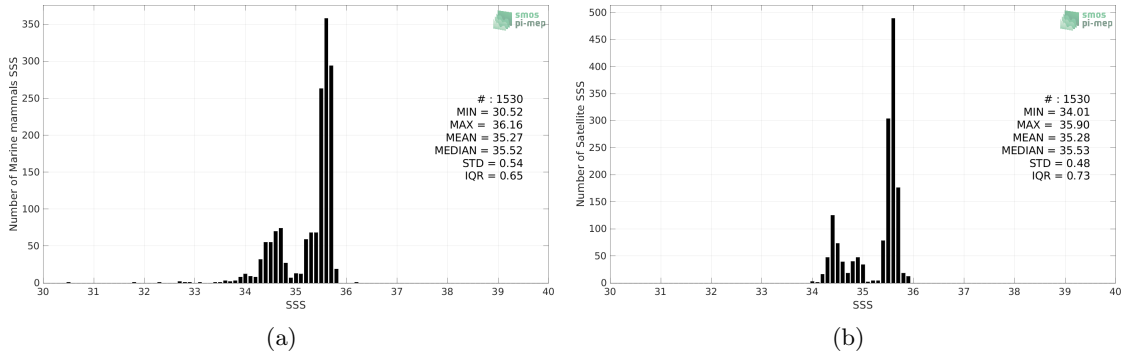
Figure 2: Histograms of SSS from Marine mammals (a) and SMAP SSS L4 OI v1 - 7 Days (IPRC) (b) considering all match-up pairs per bins of 0.1 over the South Pacific Ocean Pi-MEP region and for the full satellite product period.
