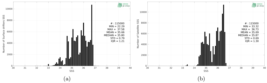
Figure 2: Histograms of SSS from Surface drifters (a) and SMAP SSS L4 OI v1 - 7 Days (IPRC) (b) considering all match-up pairs per bins of 0.1 over the South Pacific Ocean Pi-MEP region and for the full satellite product period.
