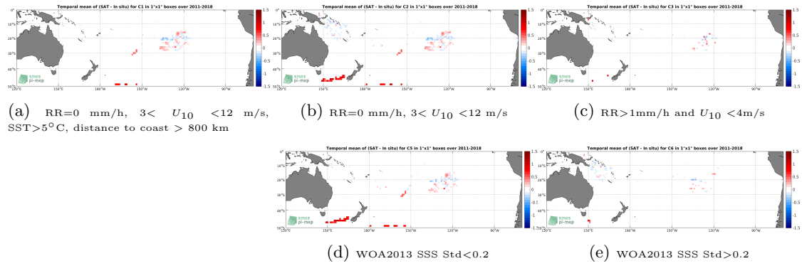
Figure 11: Temporal mean gridded over spatial boxes of size 1^\circ \times 1^\circ of \Delta SSS (SMAP SSS L4 OI v1 - 7 Days (IPRC) - Surface drifters) for 5 different subdatasets corresponding to:RR=0 mm/h, 3 < U_{10} < 12 m/s, SST >5^\circ C, distance to coast > 800 km (a), RR=0 mm/h, 3 < U_{10} < 12 m/s (b), RR >1 mm/h and U_{10} < 4 m/s (c), WOA2013 SSS Std <0.2 (d), WOA2013 SSS Std >0.2 (e).
