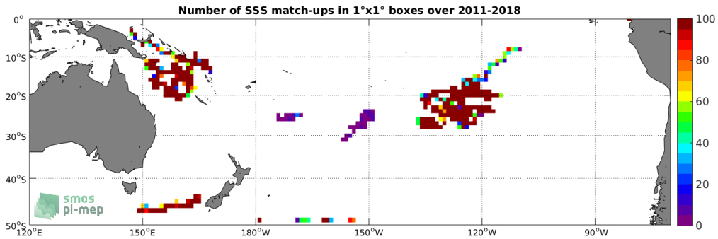
Figure 3: Number of SSS match-ups between Surface drifters SSS and the SMAP SSS L4 OI v1 - 7 Days (IPRC) SSS product for the South Pacific Ocean Pi-MEP region over 1^\circ \times 1^\circ boxes and for the full satellite product period.
