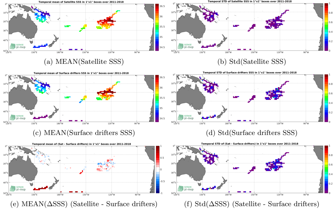
Figure 5: Temporal mean (left) and Std (right) of SSS from SMAP SSS L4 OI v1 - 7 Days (IPRC) (top), Surface drifters (middle), and of \Delta SSS (Satellite - Surface drifters). Only match-up pairs are used to generate these maps.
