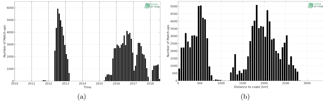
Figure 1: Number of match-ups between Surface drifters and SMAP SSS L4 OI v1 - 7 Days (IPRC) SSS as a function of time (a) and as function of the distance to coast (b) over the South Pacific Ocean Pi-MEP region and for the full satellite product period.
