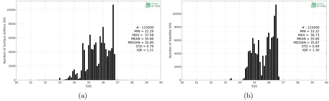
Figure 2: Histograms of SSS from Surface drifters (a) and SMAP SSS L4 OI v1 - 7 Days (IPRC) (b) considering all match-up pairs per bins of 0.1 over the South Pacific Ocean Pi-MEP region and for the full satellite product period.
