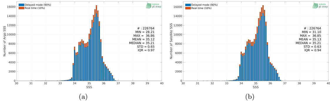
Figure 2: Histograms of SSS from Argo (a) and SMAP SSS L4 OI v1 - 7 Days (IPRC) (b) considering all match-up pairs per bins of 0.1 over the South Pacific Ocean Pi-MEP region and for the full satellite product period.
