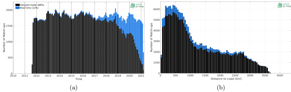
Figure 1: Number of match-ups between Argo and SMAP SSS L4 OI v1 - 7 Days (IPRC) SSS as a function of time (a) and as function of the distance to coast (b) over the South Pacific Ocean Pi-MEP region and for the full satellite product period.
