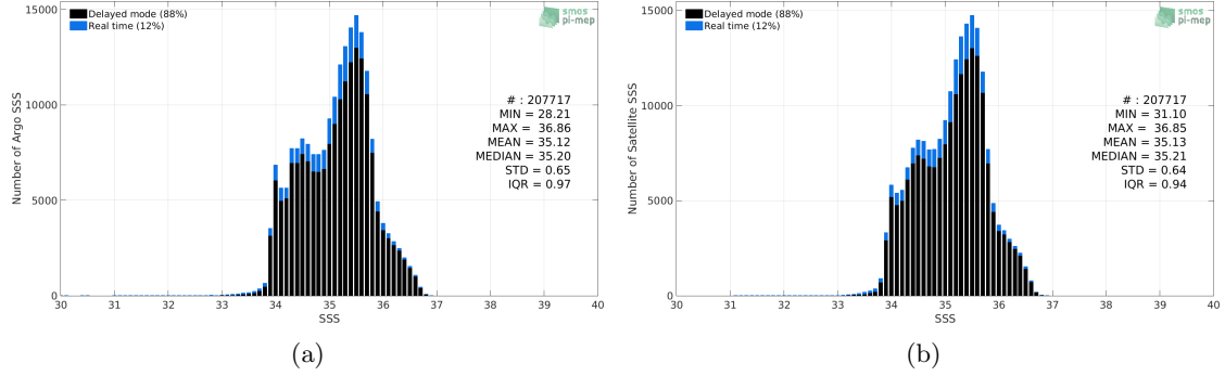
Figure 2: Histograms of SSS from Argo (a) and SMAP SSS L4 OI v1 - 7 Days (IPRC) (b) considering all match-up pairs per bins of 0.1 over the South Pacific Ocean Pi-MEP region and for the full satellite product period.
