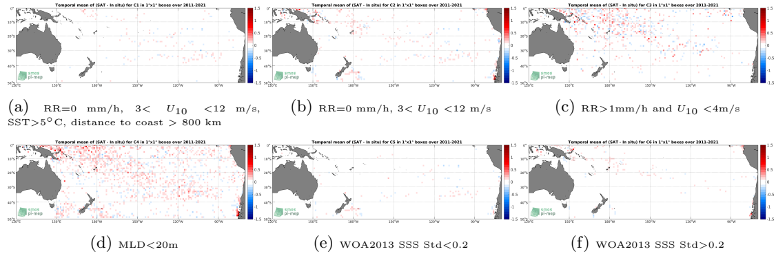
Figure 12: Temporal mean gridded over spatial boxes of size 1^\circ \times 1^\circ of \Delta SSS (SMAP SSS L4 OI v1 - 7 Days (IPRC) - Argo) for 6 different subdatasets corresponding to: RR=0 mm/h, 3 < U_{10} < 12 m/s, SST > 5^\circ C , distance to coast > 800 km (a), RR=0 mm/h, 3 < U_{10} < 12 m/s (b), RR > 1 mm/h and U_{10} < 4 m/s (c), MLD < 20 m (d), WOA2013 SSS Std < 0.2 (e), WOA2013 SSS Std > 0.2 (f).
