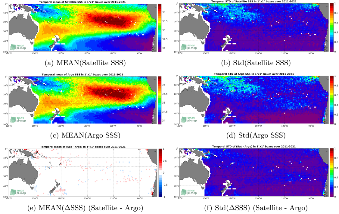
Figure 6: Temporal mean (left) and Std (right) of SSS from SMAP SSS L4 OI v1 - 7 Days (IPRC) (top), Argo (middle), and of \Delta SSS (Satellite - Argo). Only match-up pairs are used to generate these maps.
