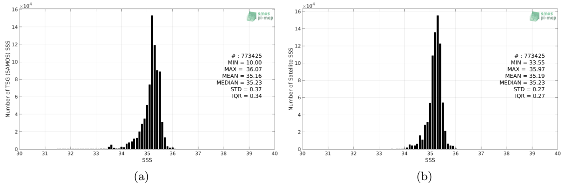
Figure 2: Histograms of SSS from TSG (SAMOS) (a) and SMAP SSS L4 OI v1 - Monthly (IPRC) (b) considering all match-up pairs per bins of 0.1 over the South Pacific Ocean Pi-MEP region and for the full satellite product period.
