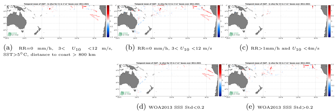
Figure 12: Temporal mean gridded over spatial boxes of size 1^\circ \times 1^\circ of \Delta SSS (SMAP SSS L4 OI v1 - Monthly (IPRC) - TSG (SAMOS)) for 5 different subdatasets corresponding to:RR=0 mm/h, 3 < U_{10} < 12 m/s, SST >5^\circ C, distance to coast > 800 km (a), RR=0 mm/h, 3 < U_{10} < 12 m/s (b), RR >1 mm/h and U_{10} < 4 m/s (c), WOA2013 SSS Std <0.2 (d), WOA2013 SSS Std >0.2 (e).
