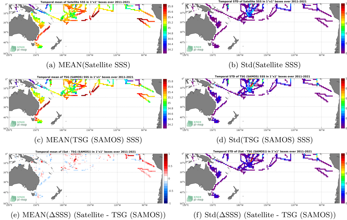
Figure 6: Temporal mean (left) and Std (right) of SSS from SMAP SSS L4 OI v1 - Monthly (IPRC) (top), TSG (SAMOS) (middle), and of \Delta SSS (Satellite - TSG (SAMOS)). Only match-up pairs are used to generate these maps.
