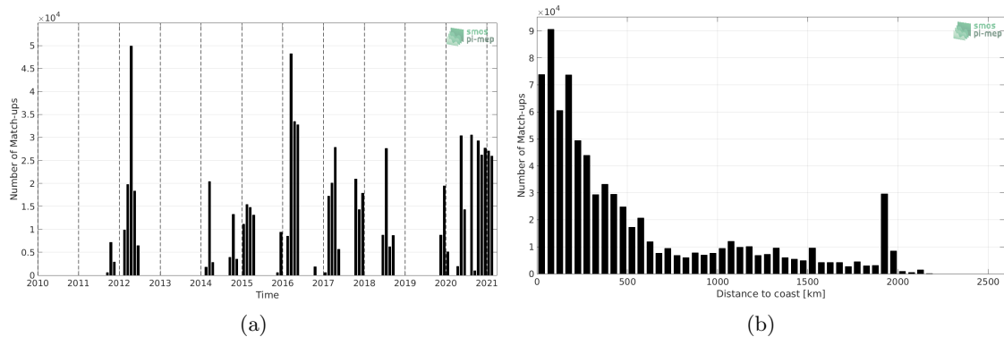
Figure 1: Number of match-ups between TSG (SAMOS) and SMAP SSS L4 OI v1 - Monthly (IPRC) SSS as a function of time (a) and as function of the distance to coast (b) over the South Pacific Ocean Pi-MEP region and for the full satellite product period.
