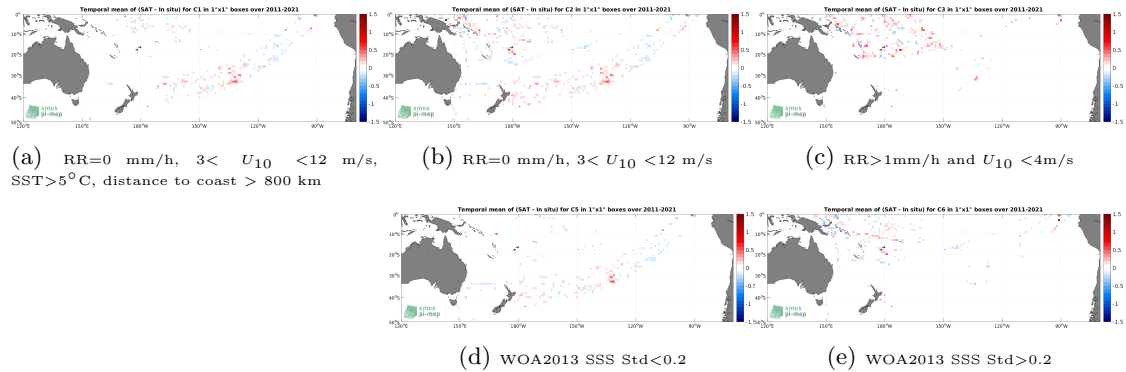
Figure 12: Temporal mean gridded over spatial boxes of size 1^\circ \times 1^\circ of \Delta SSS (SMAP SSS L4 OI v1 - Monthly (IPRC) - TSG (LEGOS-DM)) for 5 different subdatasets corresponding to:RR=0 mm/h, 3 < U_{10} < 12 m/s, SST >5^\circ\text{C} , distance to coast > 800 km (a), RR=0 mm/h, 3 < U_{10} < 12 m/s (b), RR >1 mm/h and U_{10} < 4 m/s (c), WOA2013 SSS Std <0.2 (d), WOA2013 SSS Std >0.2 (e).
