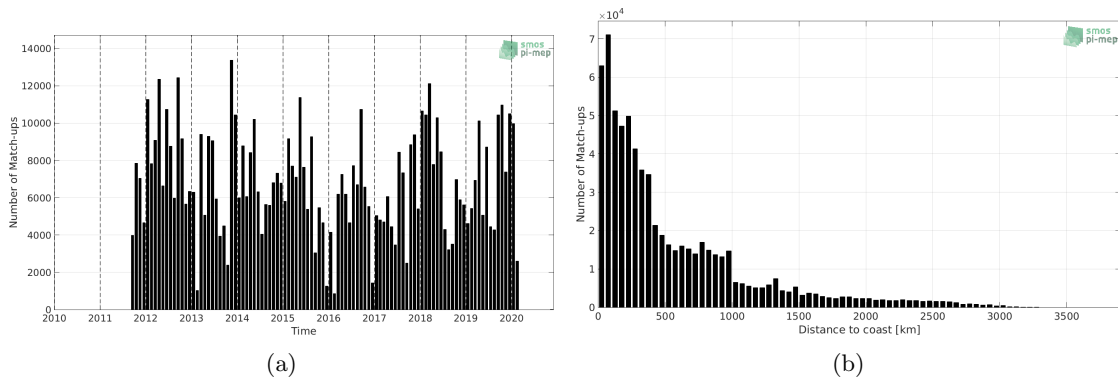
Figure 1: Number of match-ups between TSG (LEGOS-DM) and SMAP SSS L4 OI v1 - Monthly (IPRC) SSS as a function of time (a) and as function of the distance to coast (b) over the South Pacific Ocean Pi-MEP region and for the full satellite product period.
