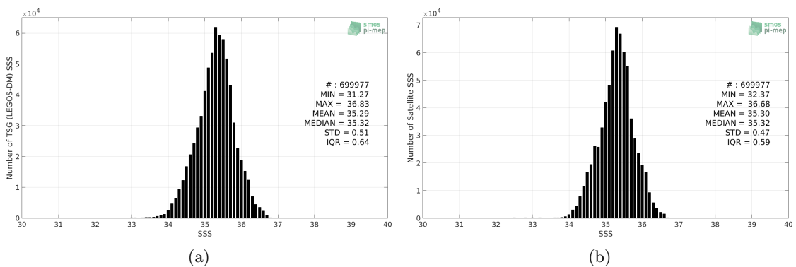
Figure 2: Histograms of SSS from TSG (LEGOS-DM) (a) and SMAP SSS L4 OI v1 - Monthly (IPRC) (b) considering all match-up pairs per bins of 0.1 over the South Pacific Ocean Pi-MEP region and for the full satellite product period.
