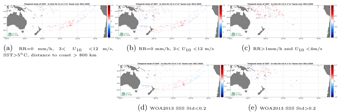
Figure 12: Temporal mean gridded over spatial boxes of size 1^\circ \times 1^\circ of \Delta\text{SSS} (SMAP SSS L4 OI v1 - Monthly (IPRC) - TSG (LEGOS-DM)) for 5 different subdatasets corresponding to:RR=0 mm/h, 3 < U_{10} < 12 m/s, SST > 5°C, distance to coast > 800 km (a), RR=0 mm/h, 3 < U_{10} < 12 m/s (b), RR > 1mm/h and U_{10} < 4 m/s (c), WOA2013 SSS Std < 0.2 (d), WOA2013 SSS Std > 0.2 (e).
