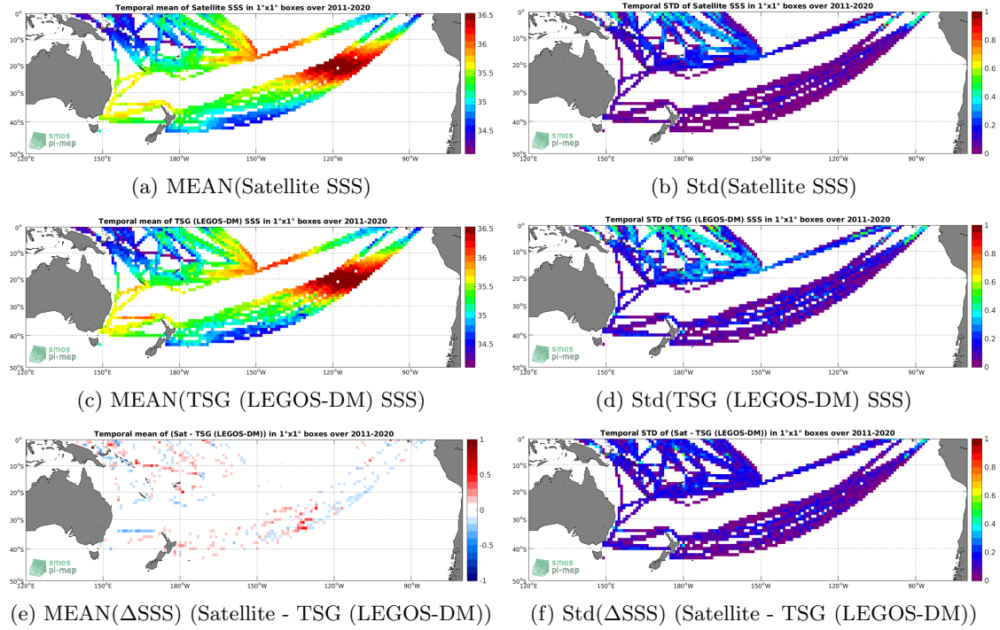
Figure 6: Temporal mean (left) and Std (right) of SSS from SMAP SSS L4 OI v1 - Monthly (IPRC) (top), TSG (LEGOS-DM) (middle), and of \Delta SSS (Satellite - TSG (LEGOS-DM)). Only match-up pairs are used to generate these maps.
