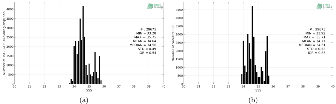
Figure 2: Histograms of SSS from TSG (GOSUD-Sailing-ship) (a) and SMAP SSS L4 OI v1 - Monthly (IPRC) (b) considering all match-up pairs per bins of 0.1 over the South Pacific Ocean Pi-MEP region and for the full satellite product period.
