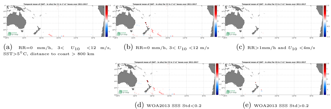
Figure 12: Temporal mean gridded over spatial boxes of size 1^\circ \times 1^\circ of \Delta\text{SSS} (SMAP SSS L4 OI v1 - Monthly (IPRC) - TSG (GOSUD-Sailing-ship)) for 5 different subdatasets corresponding to: RR=0 mm/h, 3 < U_{10} < 12 m/s, SST > 5°C, distance to coast > 800 km (a), RR=0 mm/h, 3 < U_{10} < 12 m/s (b), RR > 1mm/h and U_{10} < 4 m/s (c), WOA2013 SSS Std < 0.2 (d), WOA2013 SSS Std > 0.2 (e).
