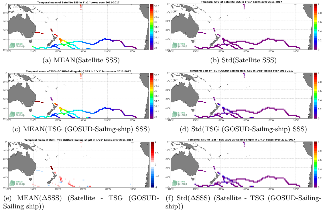
Figure 6: Temporal mean (left) and Std (right) of SSS from SMAP SSS L4 OI v1 - Monthly (IPRC) (top), TSG (GOSUD-Sailing-ship) (middle), and of \Delta SSS (Satellite - TSG (GOSUD-Sailing-ship)). Only match-up pairs are used to generate these maps.
