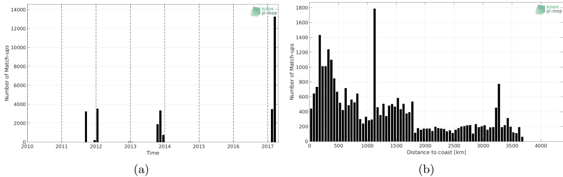
Figure 1: Number of match-ups between TSG (GOSUD-Sailing-ship) and SMAP SSS L4 OI v1 - Monthly (IPRC) SSS as a function of time (a) and as function of the distance to coast (b) over the South Pacific Ocean Pi-MEP region and for the full satellite product period.
