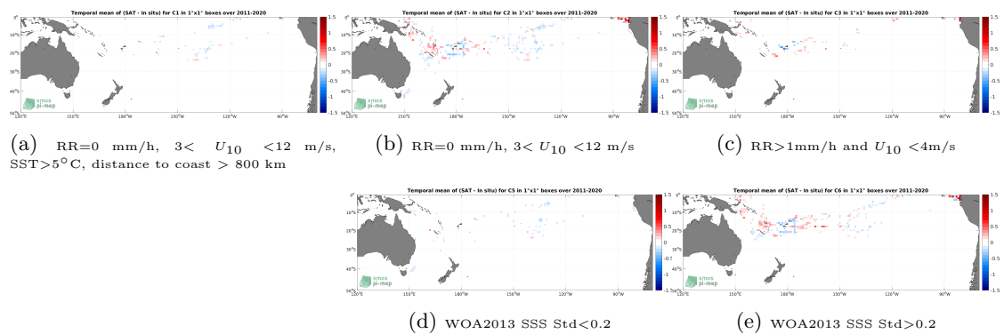
Figure 12: Temporal mean gridded over spatial boxes of size 1^\circ \times 1^\circ of \Delta SSS (SMAP SSS L4 OI v1 - Monthly (IPRC) - TSG (GOSUD-Research-vessel)) for 5 different subdatasets corresponding to:RR=0 mm/h, 3 < U_{10} < 12 m/s, SST >5^\circ\text{C} , distance to coast > 800 km (a), RR=0 mm/h, 3 < U_{10} < 12 m/s (b), RR >1 mm/h and U_{10} < 4 m/s (c), WOA2013 SSS Std <0.2 (d), WOA2013 SSS Std >0.2 (e).
