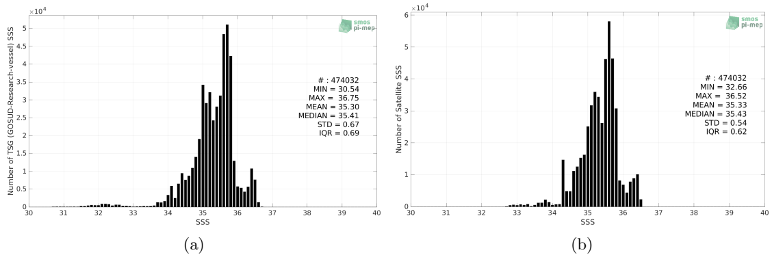
Figure 2: Histograms of SSS from TSG (GOSUD-Research-vessel) (a) and SMAP SSS L4 OI v1 - Monthly (IPRC) (b) considering all match-up pairs per bins of 0.1 over the South Pacific Ocean Pi-MEP region and for the full satellite product period.
