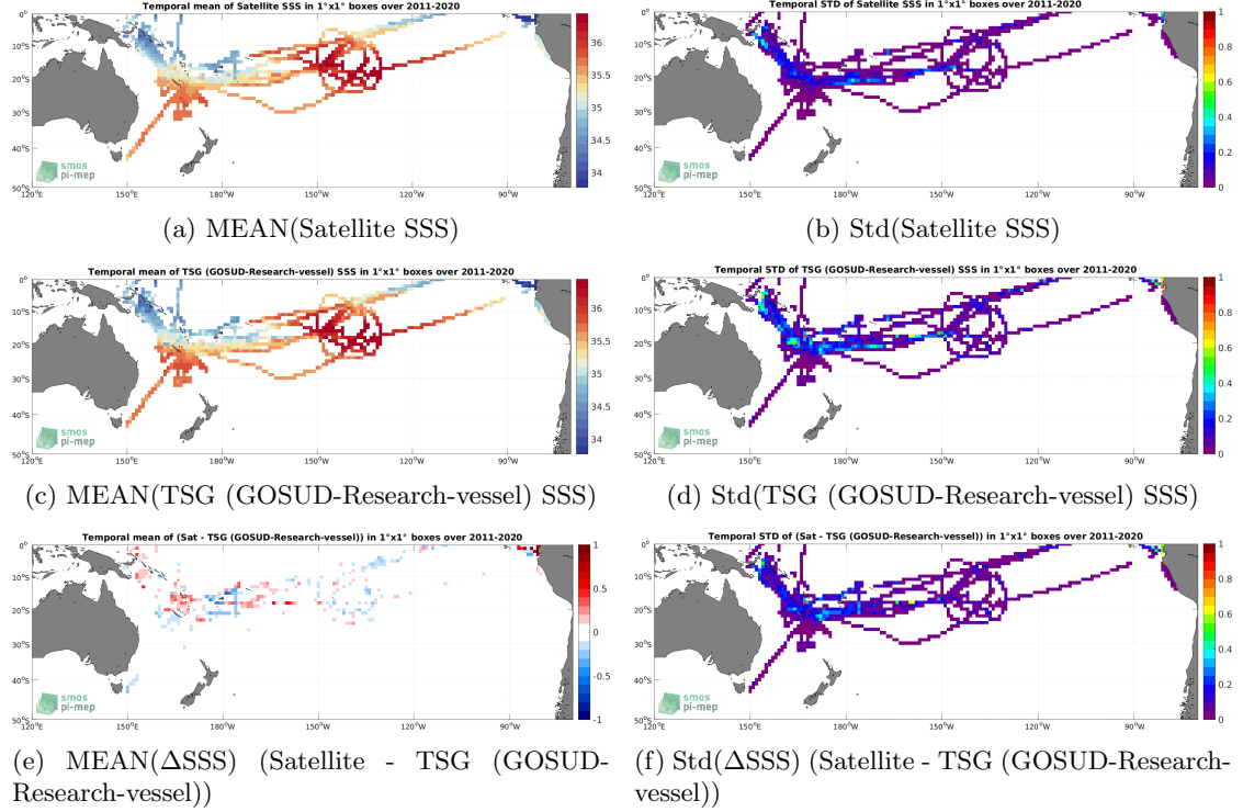
Figure 6: Temporal mean (left) and Std (right) of SSS from SMAP SSS L4 OI v1 - Monthly (IPRC) (top), TSG (GOSUD-Research-vessel) (middle), and of \Delta SSS (Satellite - TSG (GOSUD-Research-vessel)). Only match-up pairs are used to generate these maps.
