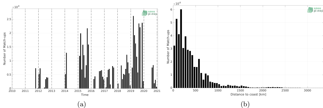
Figure 1: Number of match-ups between TSG (GOSUD-Research-vessel) and SMAP SSS L4 OI v1 - Monthly (IPRC) SSS as a function of time (a) and as function of the distance to coast (b) over the South Pacific Ocean Pi-MEP region and for the full satellite product period.
