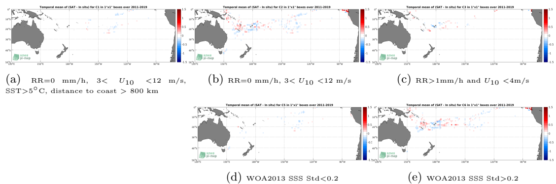
Figure 12: Temporal mean gridded over spatial boxes of size 1^\circ \times 1^\circ of \Delta\text{SSS} (SMAP SSS L4 OI v1 - Monthly (IPRC) - TSG (GOSUD-Research-vessel)) for 5 different subdatasets corresponding to: RR=0 mm/h, 3 < U_{10} < 12 m/s, SST > 5°C, distance to coast > 800 km (a), RR=0 mm/h, 3 < U_{10} < 12 m/s (b), RR > 1mm/h and U_{10} < 4 m/s (c), WOA2013 SSS Std < 0.2 (d), WOA2013 SSS Std > 0.2 (e).
