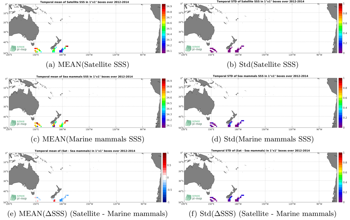
Figure 6: Temporal mean (left) and Std (right) of SSS from SMAP SSS L4 OI v1 - Monthly (IPRC) (top), Marine mammals (middle), and of \Delta SSS (Satellite - Marine mammals). Only match-up pairs are used to generate these maps.
