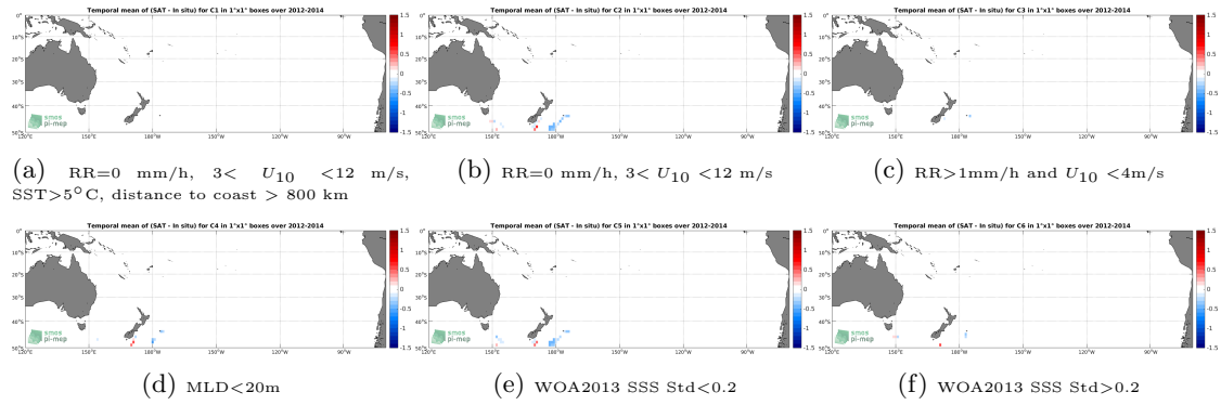
Figure 12: Temporal mean gridded over spatial boxes of size 1^{\circ}\times 1^{\circ} of \Delta\text{SSS} (SMAP SSS L4 OI v1 - Monthly (IPRC) - Marine mammals) for 6 different subdatasets corresponding to: \text{RR}=0 mm/h, 3 < U_{10} < 12 m/s, \text{SST} > 5^{\circ}\text{C} , distance to coast > 800 km (a), \text{RR}=0 mm/h, 3 < U_{10} < 12 m/s (b), \text{RR} > 1\text{mm/h} and U_{10} < 4\text{m/s} (c), \text{MLD} < 20\text{m} (d), \text{WOA2013 SSS Std} < 0.2 (e), \text{WOA2013 SSS Std} > 0.2 (f).
