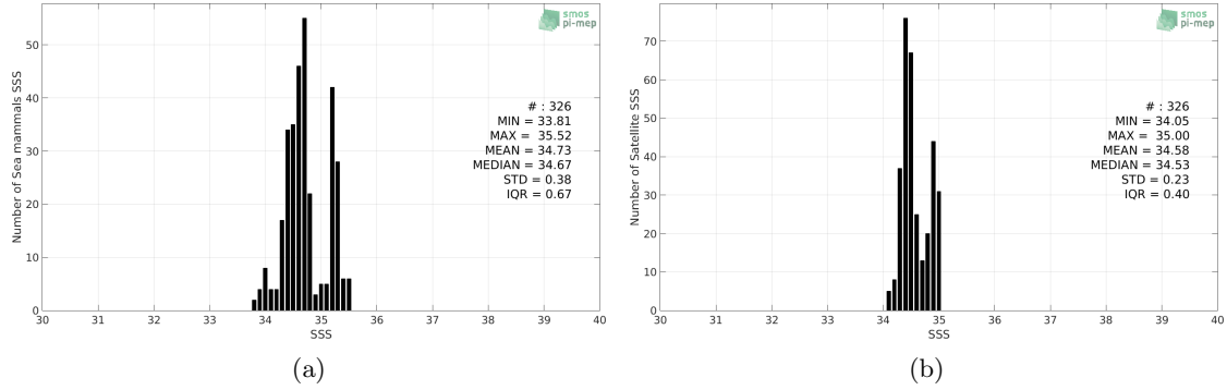
Figure 2: Histograms of SSS from Marine mammals (a) and SMAP SSS L4 OI v1 - Monthly (IPRC) (b) considering all match-up pairs per bins of 0.1 over the South Pacific Ocean Pi-MEP region and for the full satellite product period.
