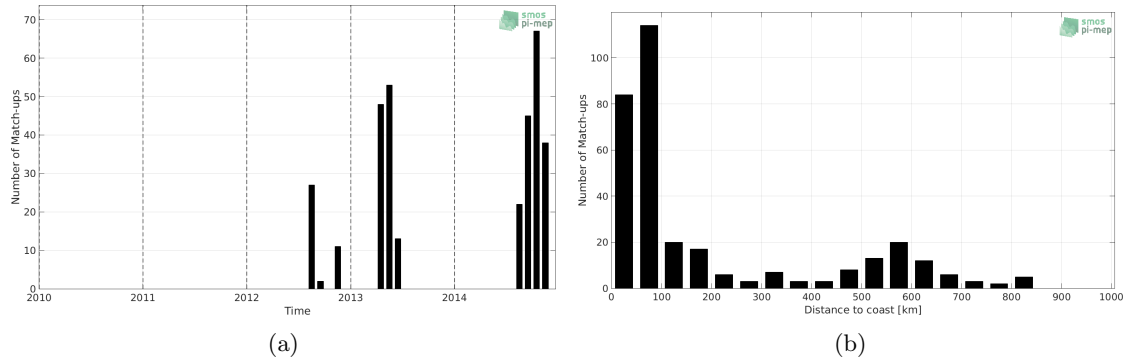
Figure 1: Number of match-ups between Marine mammals and SMAP SSS L4 OI v1 - Monthly (IPRC) SSS as a function of time (a) and as function of the distance to coast (b) over the South Pacific Ocean Pi-MEP region and for the full satellite product period.
