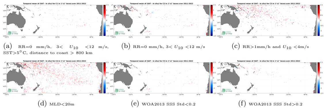
Figure 12: Temporal mean gridded over spatial boxes of size 1^\circ \times 1^\circ of \Delta SSS (SMAP SSS L4 OI v1 - Monthly (IPRC) - Argo) for 6 different subdatasets corresponding to:RR=0 mm/h, 3 < U_{10} < 12 m/s, SST >5^\circ C, distance to coast > 800 km (a), RR=0 mm/h, 3 < U_{10} < 12 m/s (b), RR >1 mm/h and U_{10} < 4 m/s (c),MLD <20 m (d),WOA2013 SSS Std <0.2 (e),WOA2013 SSS Std >0.2 (f).
