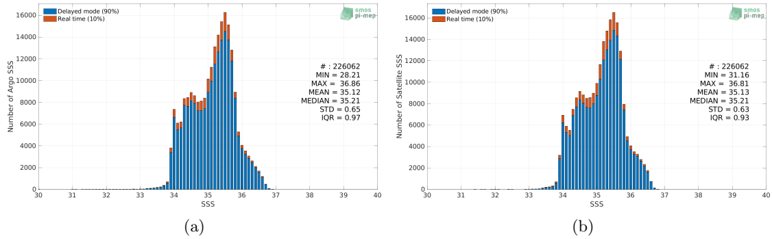
Figure 2: Histograms of SSS from Argo (a) and SMAP SSS L4 OI v1 - Monthly (IPRC) (b) considering all match-up pairs per bins of 0.1 over the South Pacific Ocean Pi-MEP region and for the full satellite product period.
