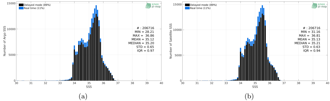
Figure 2: Histograms of SSS from Argo (a) and SMAP SSS L4 OI v1 - Monthly (IPRC) (b) considering all match-up pairs per bins of 0.1 over the South Pacific Ocean Pi-MEP region and for the full satellite product period.
